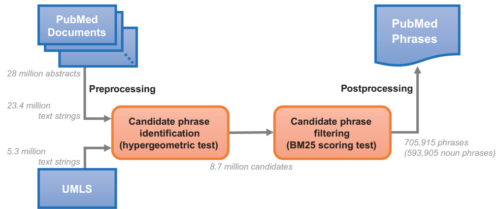
Figure 1. Workflow of PubMed Phrase extraction.
