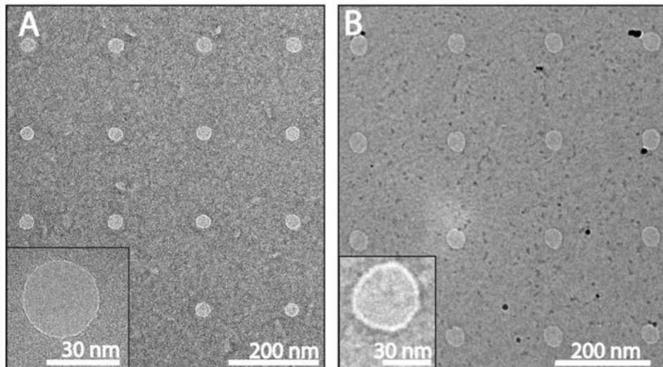
Figure 2. TEM image of nanopore arrays fabricated using RIE
