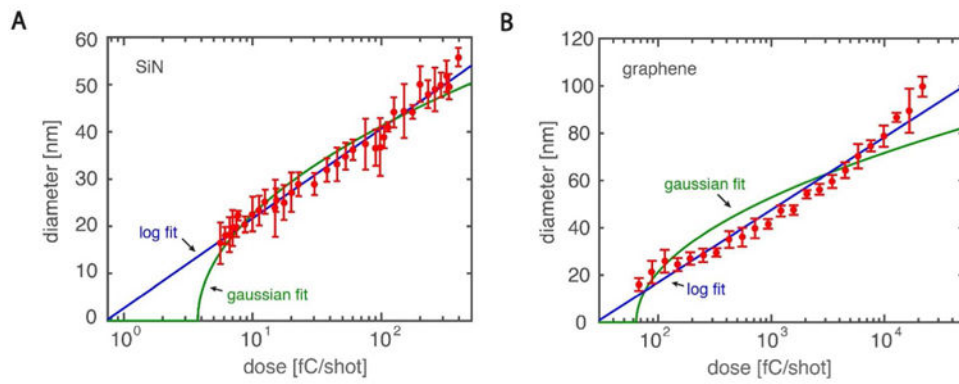
Figure 3. Single-shot nanopore diameter versus electron-beam dose
