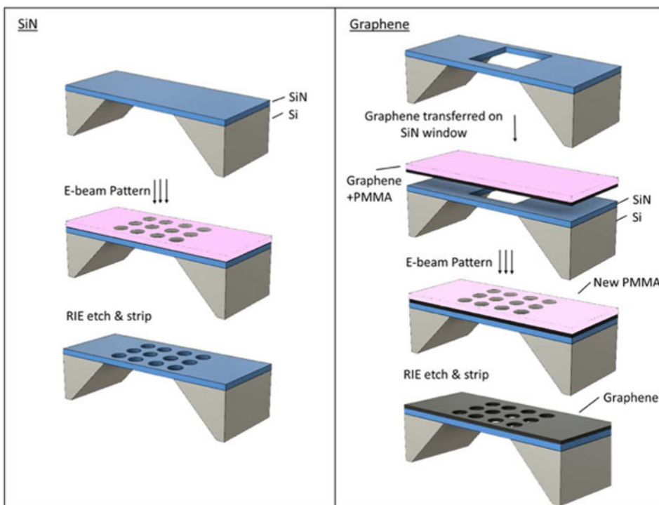
Figure 1. Schematic of EBL assisted RIE nanopore fabrication
