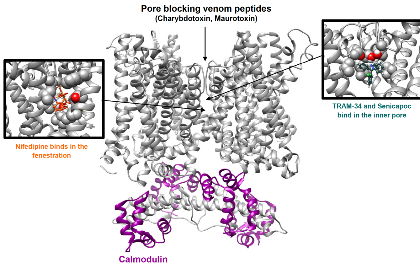
Fig. (2). Cartoon illustrating the binding sites of the triarylmethanes TRAM-34 and senicapoc in the inner pore and nifedipine in the fenestration region of K_{Ca3.1} . The tetramer of K_{Ca3.1} alpha-subunits is shown as a grey ribbon. The channel associated calmodulin is shown in dark magenta. (The color version of the figure is available in the electronic copy of the article).
