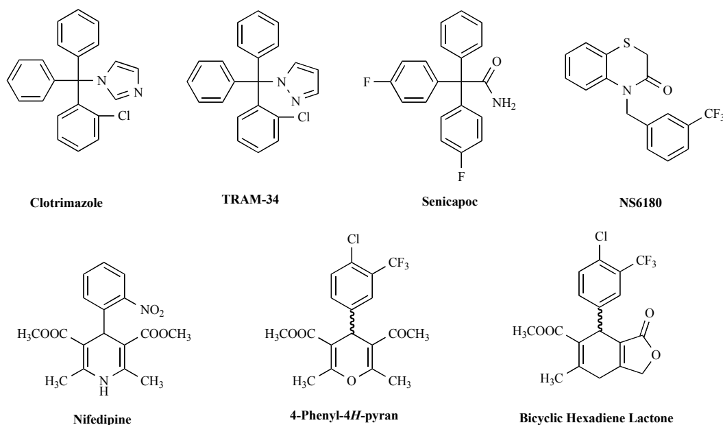
Fig. (1). Chemical structures of K_{Ca3.1} inhibitors.
