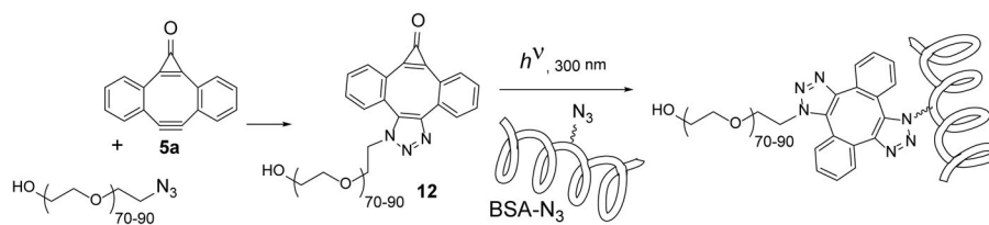
Scheme 8. PEGylation of BSA
