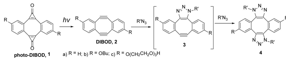
Scheme 1. Azide cross-linking using bis-caged dibenzo[ a, e ]cyclooctyne
