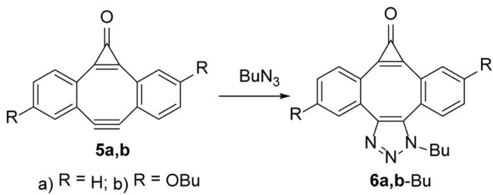
Scheme 4. SPAAC of butyl azide across the triple bond of MC-DIBOD (5)
