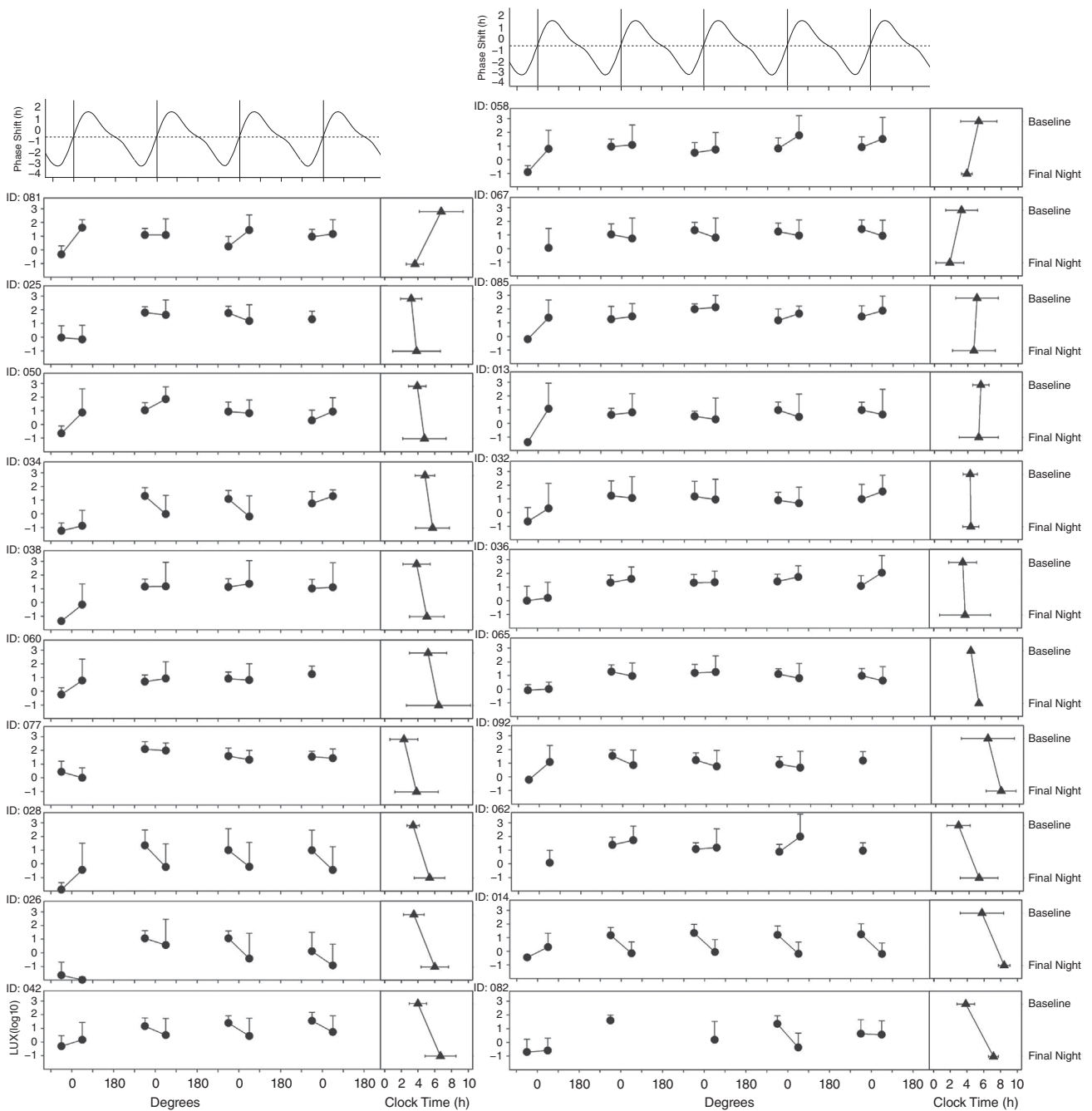
Figure 3. Light exposure relative to circadian phase for each participant The circles represent log 10 lux averaged in each delay (90 degs before acrophase) and advance (90 degs after acrophase) zone at baseline, first night shift (N1), second night shift (N2), third night shift (N3) and fourth night shift (N4). Light is averaged relative to individual circadian phase: the x-axis represents circadian degrees (360 deg = 24+daily phase shift), such that 0 indicates acrophase each day. Triangles represent aMT6s acrophase in clock time at baseline and final night shift (error bars show 95% confidence intervals). The difference between light in delay compared to advance zones was examined at baseline and each night shift to examine the relationship with the direction of phase shift for each participant.
