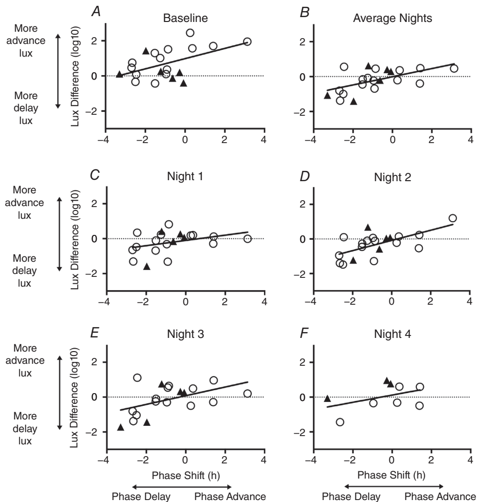
Figure 4. Relationship between phase shift and the difference between delay and advance light in the 90 deg either side of acrophase time at baseline, first night shift (N1), second night shift (N2), third night shift (N3), fourth night shift (N4) and averaged over all night shifts (Mean Night)
