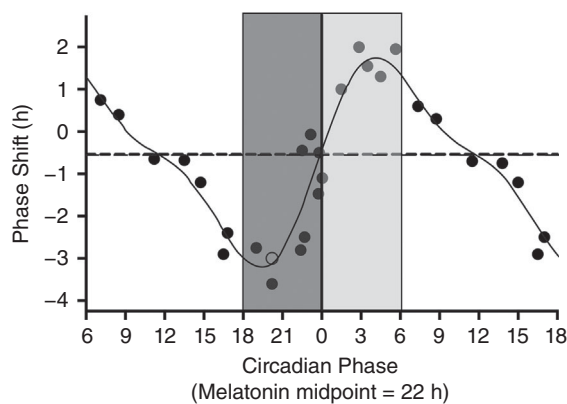
Figure 1. Phase response curve to light (adapted from Khalsa et al. 2003), where 0 on the abscissa represents timing of core body temperature minimum (CBTmin) in healthy subjects
