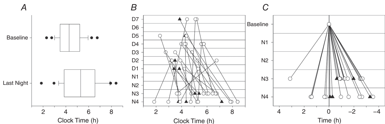
Figure 2. aMT6s acrophase over the shift schedule
