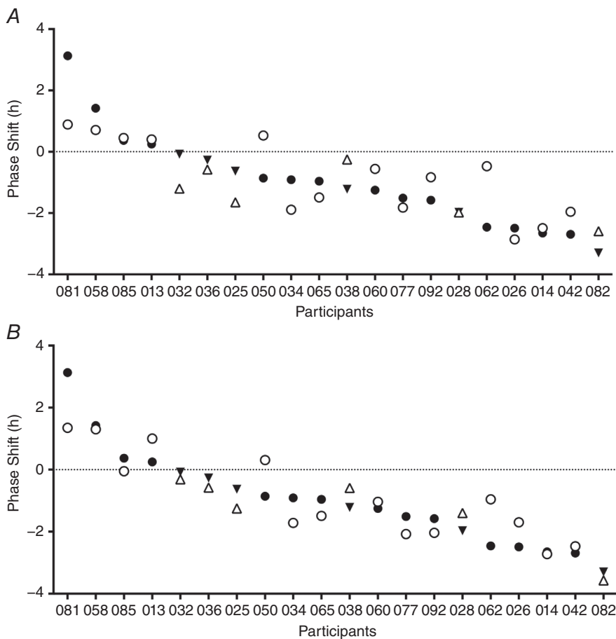
Figure 5. Predicted vs. actual phase shift for each participant from two models
