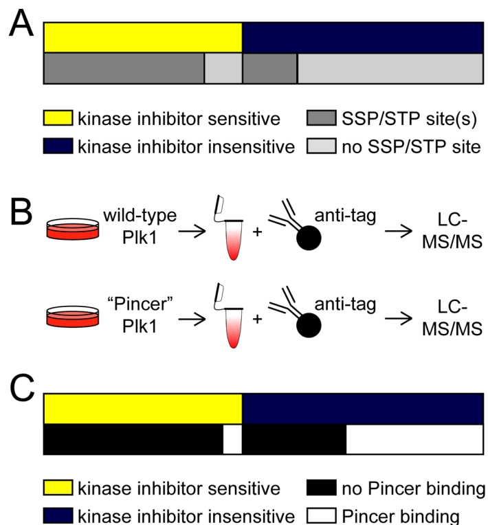
Figure 3. Stable interactors of Plk1 include phosphorylation-dependent interactions
