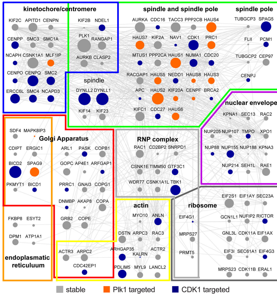
Figure 2. Subcellular localization map of Plk1 interactors
