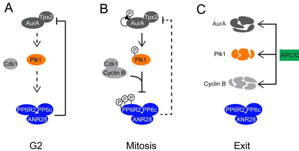
Figure 7. Model of regulatory feedback governing Aurora A, Plk1 and PP6
