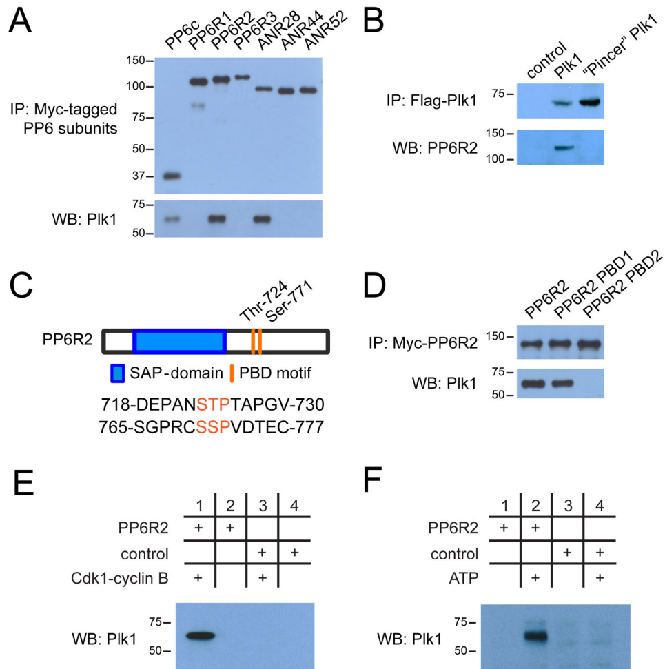
Figure 4. Regulatory interaction of PP6 and Plk1
