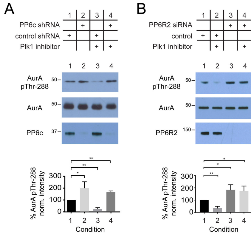
Figure 6. Regulation of PP6 phosphatase activity by Plk1 in cells (A and B) Representative Western blot and analysis of total and phosphorylated (Thr 288 ) Aurora A upon depletion of PP6c (A) or PP6R2 (B), Plk1 inhibition with BI2536, or both. Data are mean ± S.D. of 3 biological replicates; * p < 0.05, ** p < 0.01).
