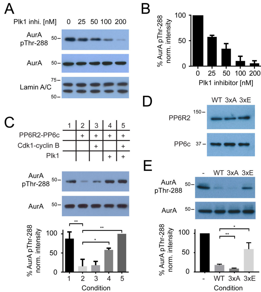
Figure 5. Regulation of PP6 phosphatase activity by Plk1 in vitro
