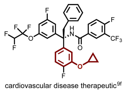
Figure 2. Representative bioactive compounds bearing cyclopropylaryl ethers. [9]
