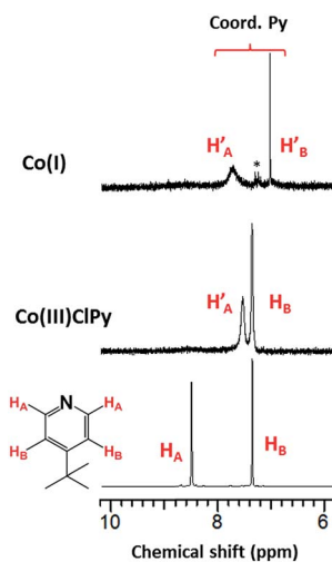
Fig. 11 1 H-NMR spectra of [Co I (prdioxH)( 4t Bu 4 py)], in CD 3 CN. The asterisk denotes the presence of adventitious toluene. See ESI† for the complete spectra.
