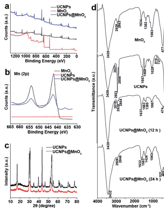
Fig. 3 (a) XPS spectra of UCNPs, \text{MnO}_2 and UCNPs@ \text{MnO}_2 . (b) High resolution Mn ( 2p ) XPS spectra of UCNPs, \text{MnO}_2 and UCNPs@ \text{MnO}_2 . (c) XRD spectra of UCNPs and UCNPs@ \text{MnO}_2 . (d) FT-IR spectra of \text{MnO}_2 , UCNPs, and UCNPs@ \text{MnO}_2 at different oxidation times ( 12 \text{ h} and 24 \text{ h} ).
