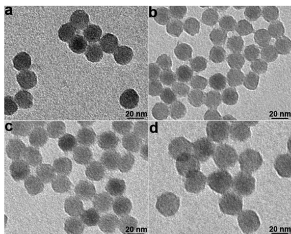
Fig. 2 TEM images of the oxidized UCNPs from the experimental group at different times. (a) 2 \text{ h} ; (b) 6 \text{ h} ; (c) 12 \text{ h} ; (d) 24 \text{ h} .
