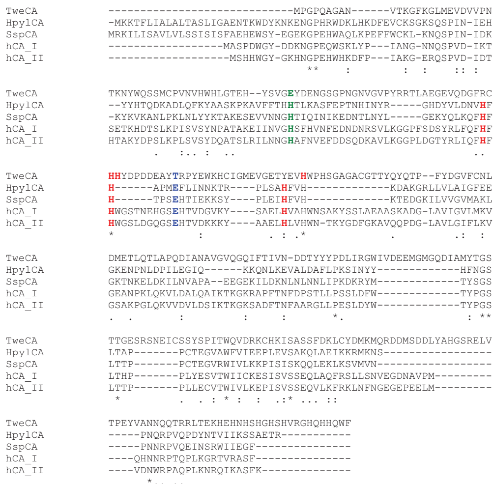
Figure 3. Multialignment of the TweCA \delta amino acid sequence with those of bacterial (Hpy1CA, \alpha -CA from Helicobacter pylori , SspCA, \alpha -CA from Sulfurihydrogenibium yellowstonensis ) and human (hCA I and II) \alpha -class enzymes. The zinc ligands of the \alpha -CAs and the putative zinc ligands of TweCA \delta are evidenced in red, whereas amino acid residues involved in the catalytic inhibition/mechanism (e.g. His64 and Asp106, hCA I numbering) are shown in green and blue, respectively.
