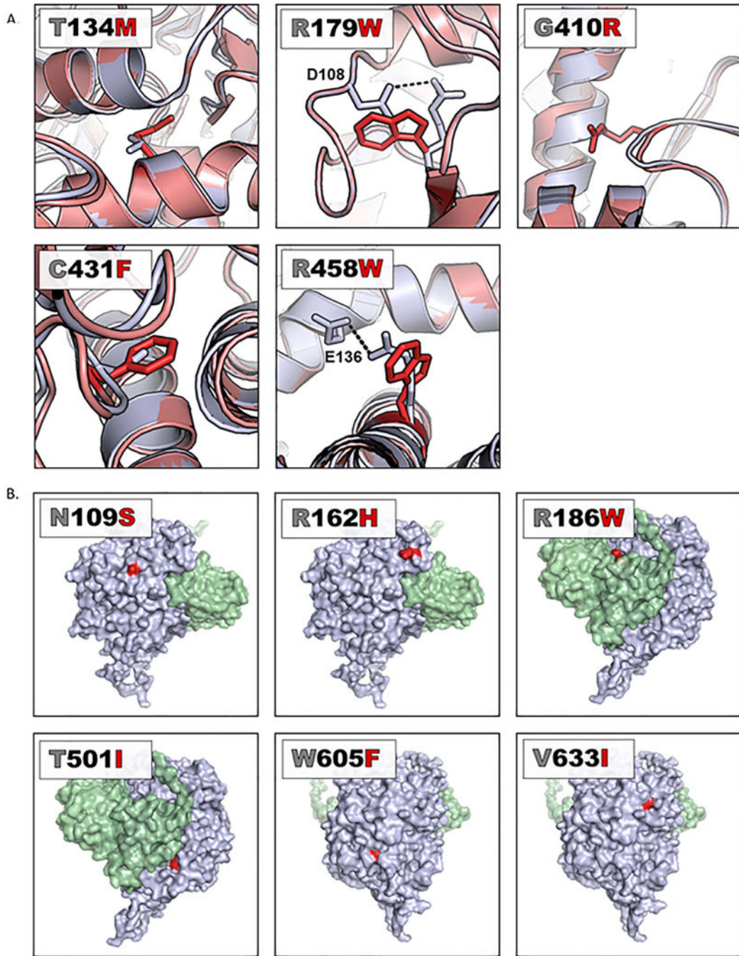
Figure 4. Structural consequences of variants visualized in a yeast model (yeast model PDB file 1ORZ)
