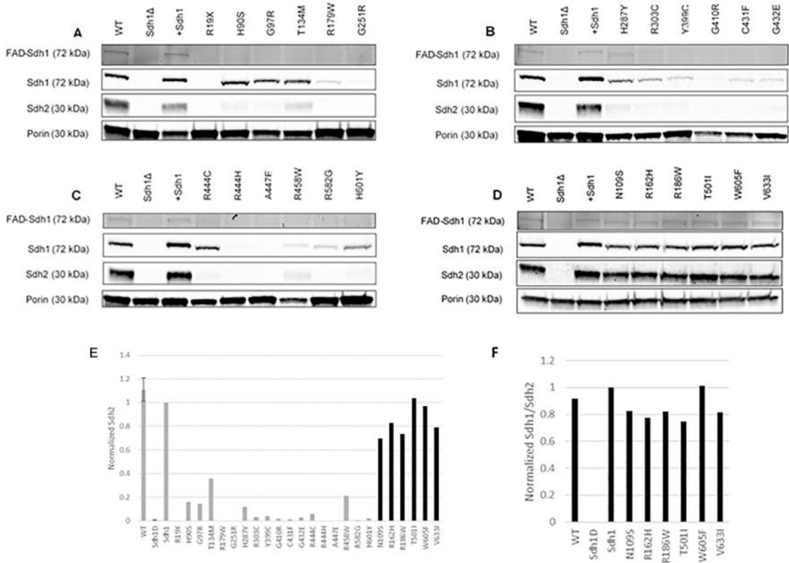
Figure 2. Abundance of flavinated Sdh1, total Sdh1, and total Sdh2 in mitochondrial lysates from yeast expressing each variant
