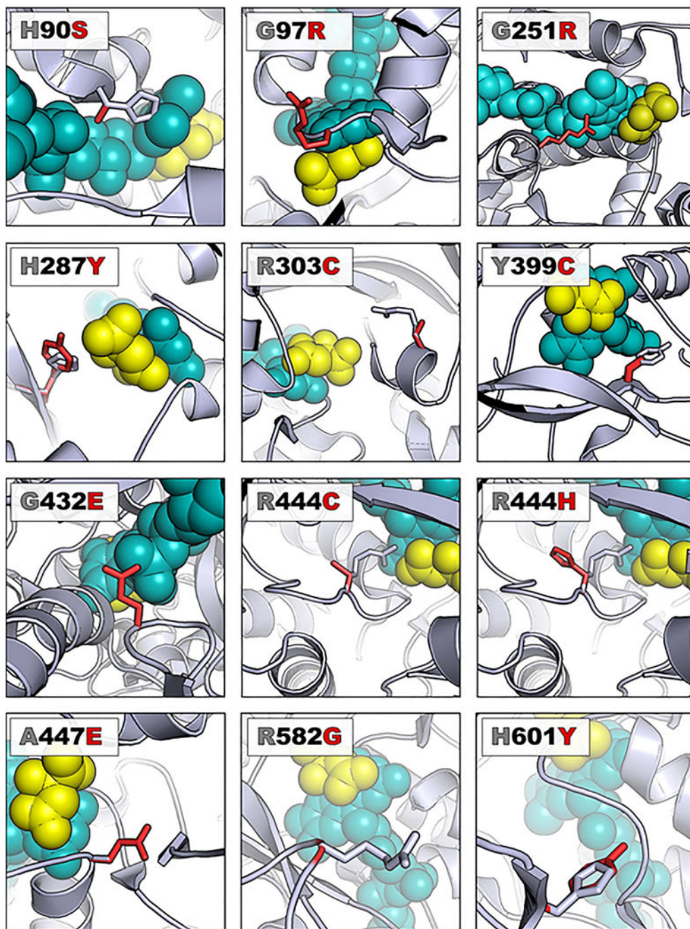
Figure 3. Variants involving the active site cause loss of Sdh1 function
