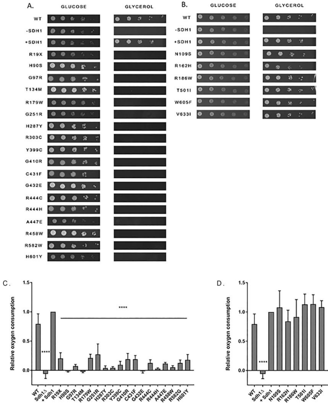
Figure 1. ySdh1 variants causing loss of function are unable to use glycerol as a sole carbon source or consume oxygen
