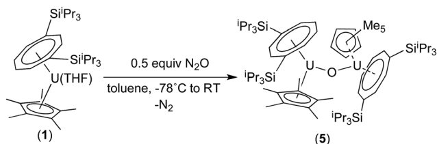
Scheme 2 Synthesis of (5).
