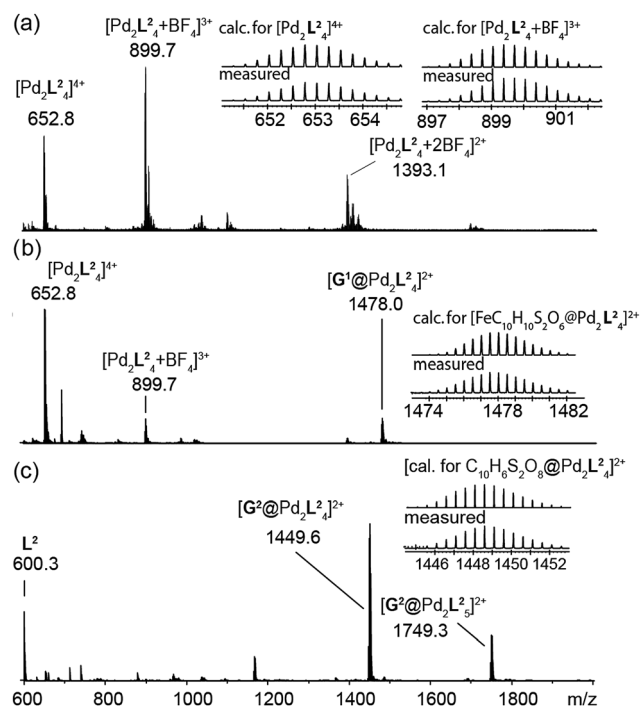
Fig. 3 ESI mass spectra of the cage and some host-guest complexes. (a) [\text{Pd}_2\text{L}_4] , (b) [\text{G}^1@Pd_2\text{L}_4] , and (c) [\text{G}^2@Pd_2\text{L}_4] .
