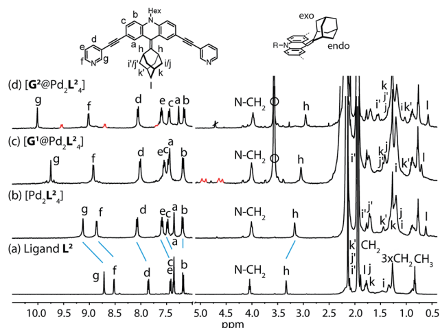
Fig. 2 ^1\text{H} NMR spectra of the cage and some host-guest complexes. (a) Ligand \text{L}^2 , (b) cage [\text{Pd}_2\text{L}_4] , (c) [\text{G}^1@Pd_2\text{L}_4] , and (d) [\text{G}^2@Pd_2\text{L}_4] (400 MHz, 298 K, \text{CD}_3\text{CN} ). The signals of the encapsulated guest molecules are highlighted in red. \text{H}_i , \text{H}_j and \text{H}_k represent outside ( exo ) and \text{H}_i' , \text{H}_j' and \text{H}_k' inside ( endo ) pointing hydrogen atoms of the adamantyl substituent with respect to the acridone backbone (compare Fig. 4a). Empty circle: [\text{K}(\text{18-crown-6})]^+ .
