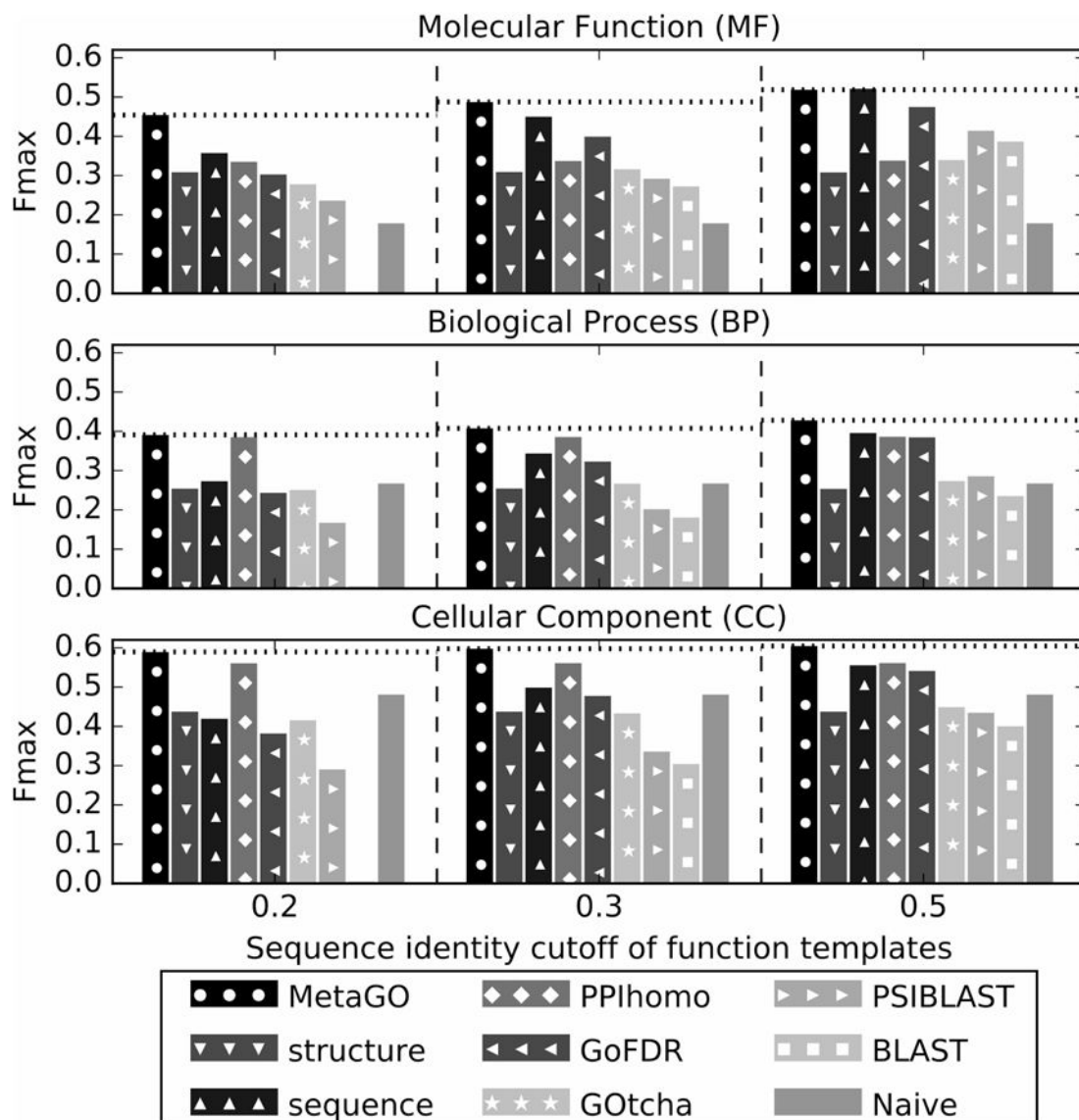
Figure 2. Fmax score of the GO predictions by MetaGO, compared to that by the three component pipelines (structure, sequence, and PPI-homolog), and four control methods (GoFDR, GOTcha, BLAST, PSI-BLAST, and Naïve) at different sequence identity cut-offs for filtering functional templates. The dotted lines label the performance of MetaGO. A color version of this figure is provided as Figure S2 in Supplemental Material.
