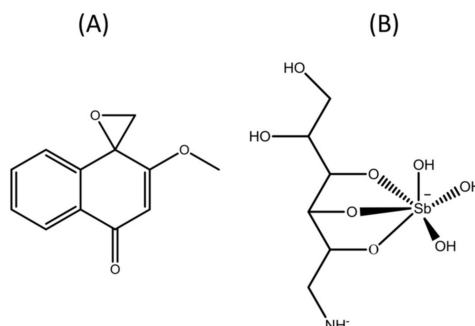
Figure 1. Chemical structure of drugs. (A) 2-methoxy-4H-spiro[naphthalene-1,2'-oxiran]-4-one, also known as Epoxymethoxy-lawsone ( C_{12}H_{10}O_3 , 202.21 g/mol) and (B) meglumine antimoniate known commercially as Glucantime ® ( C_7H_{18}NO_8Sb , 365.98 g/mol—structure proposed by Frézard et al. [15]).
