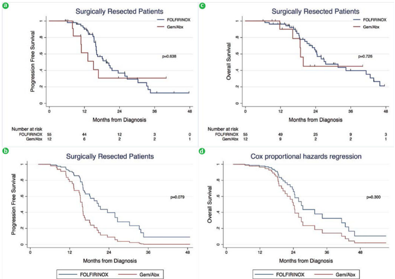
Figure 2. (a). PFS among surgically resected patients on unadjusted and (b). adjusted analysis. (c). OS among surgically resected patients on unadjusted and (d). adjusted analysis. Gem-Abx gemcitabine and abraxane
