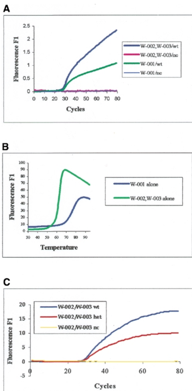
Figure 3. (A) PCR amplification. The fluorescent signal for the duplex Scorpion/quencher pair W-002/W-003 is higher than for the stem-loop Scorpion W-001 (proportional mode). (B) Fluorescence melting curves of stem-loop (W-001) and duplex (W-002/W-003) Scorpion oligonucleotides. (C) Allelic discrimination using the duplex Scorpion/quencher W-002/W-003. Fluorescence for the wild-type template is almost double that of the heterozygote (arithmetic mode). wt, wild-type template; het, heterozygote; nc, negative control.
