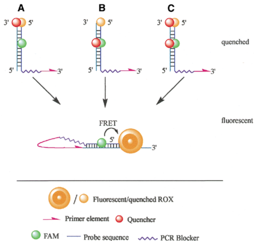
Figure 5. FRET duplex Scorpions with three different versions of the quencher oligonucleotide.
