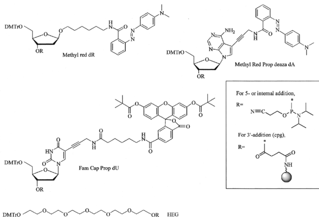
Figure 2. Chemical structures of non-standard monomers.
