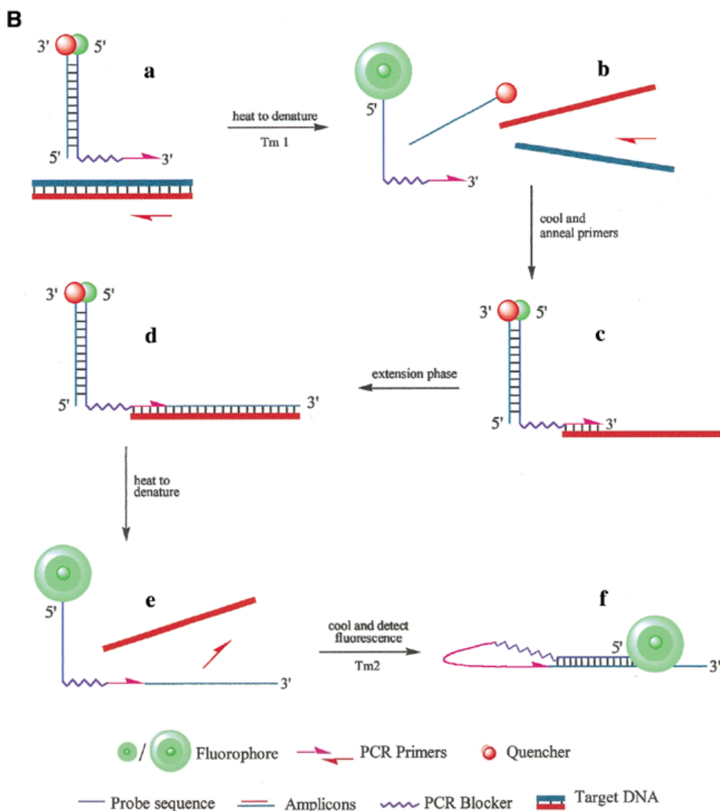
Figure 1. (A) (Previous page) The stem-loop Scorpion format in PCR. On cooling, after PCR primer extension, the probe element binds to its complement on the same strand and fluorescence is observed (structure f). (B) The duplex Scorpion format. The unimolecular probing mechanism is basically the same as in the stem-loop format. Fluorescence of structure f is measured during PCR. wt, wild-type template; het, heterozygote; mut, homozygote mutant; nc, negative control.
