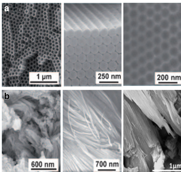
Fig. 3 SEM images of anodized \text{TiO}_2 nanotube layers by different anodization processes of Ti. a The highly ordered \text{TiO}_2 nanotubes (in top and side view) are obtained in organic electrolyte systems, with self-ordered surface dimples (right) which in fact are metallic surfaces when the tube layers are removed. Reproduced from ref. [1]. b The disordered \text{TiO}_2 nanotubes are grown in patches on the surface area and fused together to bundles in chloride containing electrolyte by an ultrafast anodization technique known as rapid-breakdown anodization (RBA). Reproduced from ref. [1] and [37]
