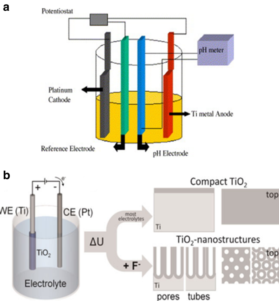
Fig. 2 Schematic set up. a Illustrative drawing of a three-electrode system with the prepared Ti foil as the working electrodes, platinum as the counter electrode, and usually Ag/AgCl as a reference electrode, while the pH electrode as a pH meter. Reproduced from ref. [35]. b Illustrative drawing of a simple two-electrode system composed of Ti foil as anode and inert metal electrode as cathode. Anodization leads to different anodized oxide layer under different conditions. In most neutral and acidic electrolytes, a compact titania can be formed. But if dilute fluoride electrolytes are used, nanotubular/nanoporous oxide layers will be directly attached to the metal surface. Reproduced from ref. [36]
