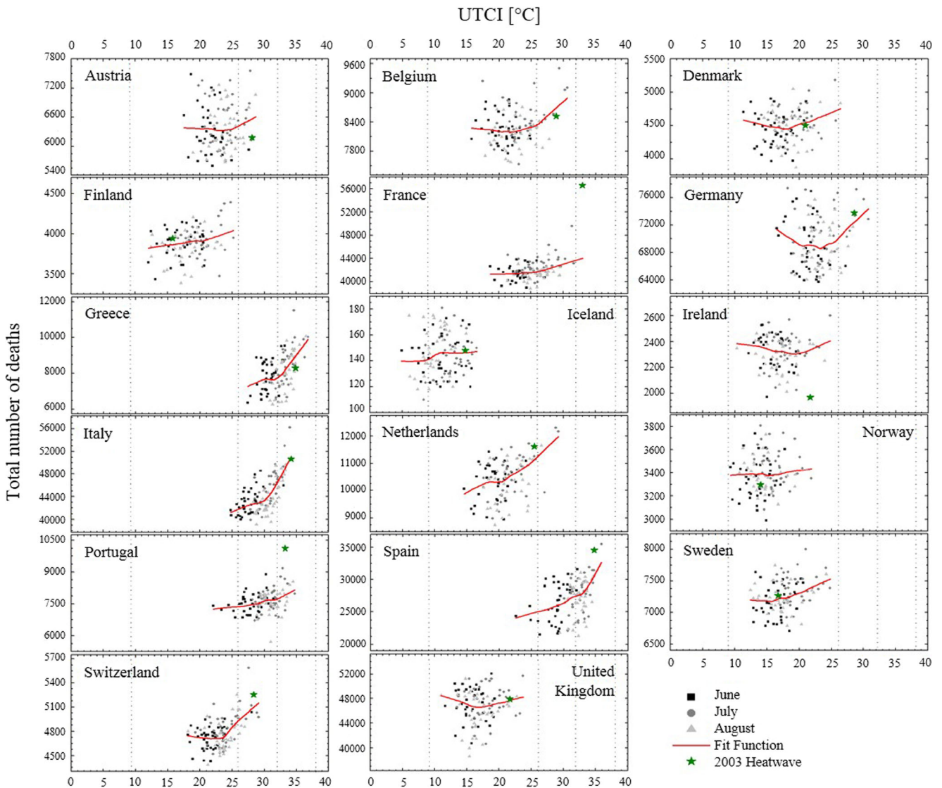
Fig. 4 Scatter diagrams for monthly number of all-cause deaths and monthly average of UTCI daily maximum values per European country for the 1979–2015 period. Dashed lines delimitate UTCI stress categories
