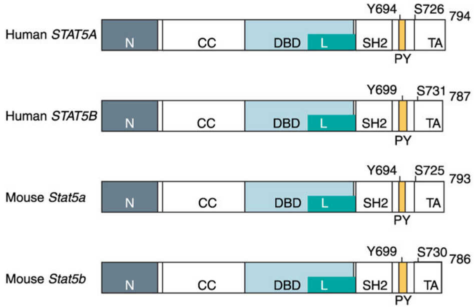
Figure 1. The major structural and functional domains and the phosphorylation sites of human and mouse STAT5A and STAT5B proteins. STAT5 proteins share an overall general structure that is organized into functional modular domains: N-terminal domain (N), coiled-coil domain (CC), DNA-binding domain (DBD), linker domain (L), SH2 domain (SH2), and transactivation domain (TA). All STAT molecules have a highly conserved tyrosine phosphorylation site (Y) at or around residue 700, labeled as the phosphotyrosyl segment (PY). Tyrosine phosphorylation follows ligand-induced activation and is required for dimerization and nuclear translocation.
