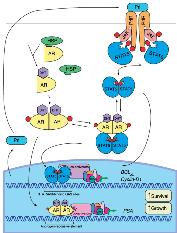
Figure 2. Functional interaction between JAK2-STAT5A/B and androgen receptor (AR) signaling in prostate cancer cells. Binding of prolactin (PRL) to prolactin receptor (PRLR) results in receptor dimerization and activates the receptor associated kinase, Janus kinase 2 (JAK2). JAK2 phosphorylates the PRLR on tyrosine residues, thereby creating docking sites for the SH2 domain of STAT5A/B monomers. STAT5A/B molecules are phosphorylated on unique tyrosine residues by JAK2, dissociate from the receptors, dimerize, and translocate to the nucleus where they bind to specific STAT5A/B-binding GAS ( \gamma -interferon activation sequence) sites within the promoters of target genes. Binding of androgens (DHT) to the androgen receptor (AR) induces the dissociation from heat shock proteins (HSPs), receptor phosphorylation, and dimerization. Dimerized AR is translocated into the nucleus and bind to androgen response elements at the promoter of target genes. In prostate cancer cells, liganded AR interacts with activated STAT5A/B and enhances the nuclear translocation STAT5A/B. STAT5A/B, in turn, increases the nuclear translocation of AR. STAT5A/B and AR are both growth promoting signaling pathways in prostate cancer cells.
