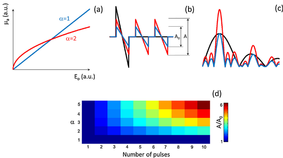
Fig. 2. Effects of optical absorption saturation on optoacoustic signals generated with tone-burst excitation. (a) Absorption coefficient as a function of optical energy modelled as \mu_a = kE_{o1}^{1/\alpha} , where \alpha = 1 corresponds to the linear optoacoustic signal generation regime. (b) Optoacoustic signals generated for single pulse excitation (black) versus tone-burst of 3 pulses with the same total energy for \alpha = 1 (blue) and \alpha = 2 (red). (c) The corresponding frequency spectra of the signals. (d) Amplitude of the optoacoustic signals generated with the tone-burst excitation normalized to the signal generated with a single pulse with the same total energy.
