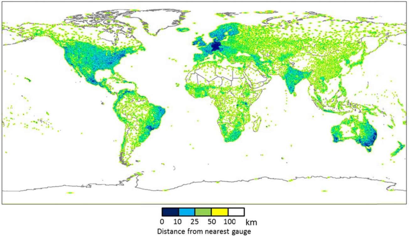
Figure 2. Map showing the distance to nearest GPCC gauge, typical of all regular and reliable gauge measurements; blank areas in the figure are beyond 100 km from the nearest gauge.
