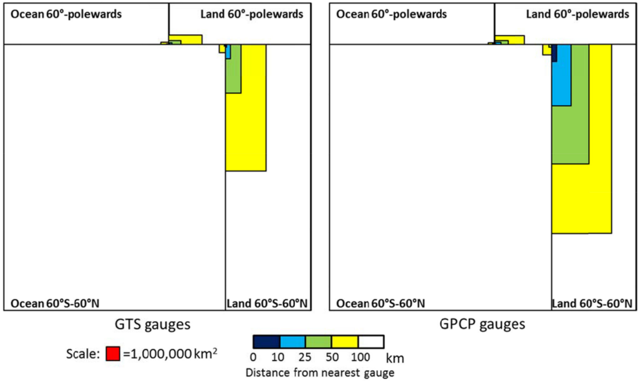
Figure 4. Areas of the Earth within certain distances from the nearest precipitation gauge for the GTS network (left) and the GPCP dataset (right). The whole square represents the whole of the Earth's surface, while the subdivisions are for land and ocean and 60°-polewards and 60°S–60°N.
