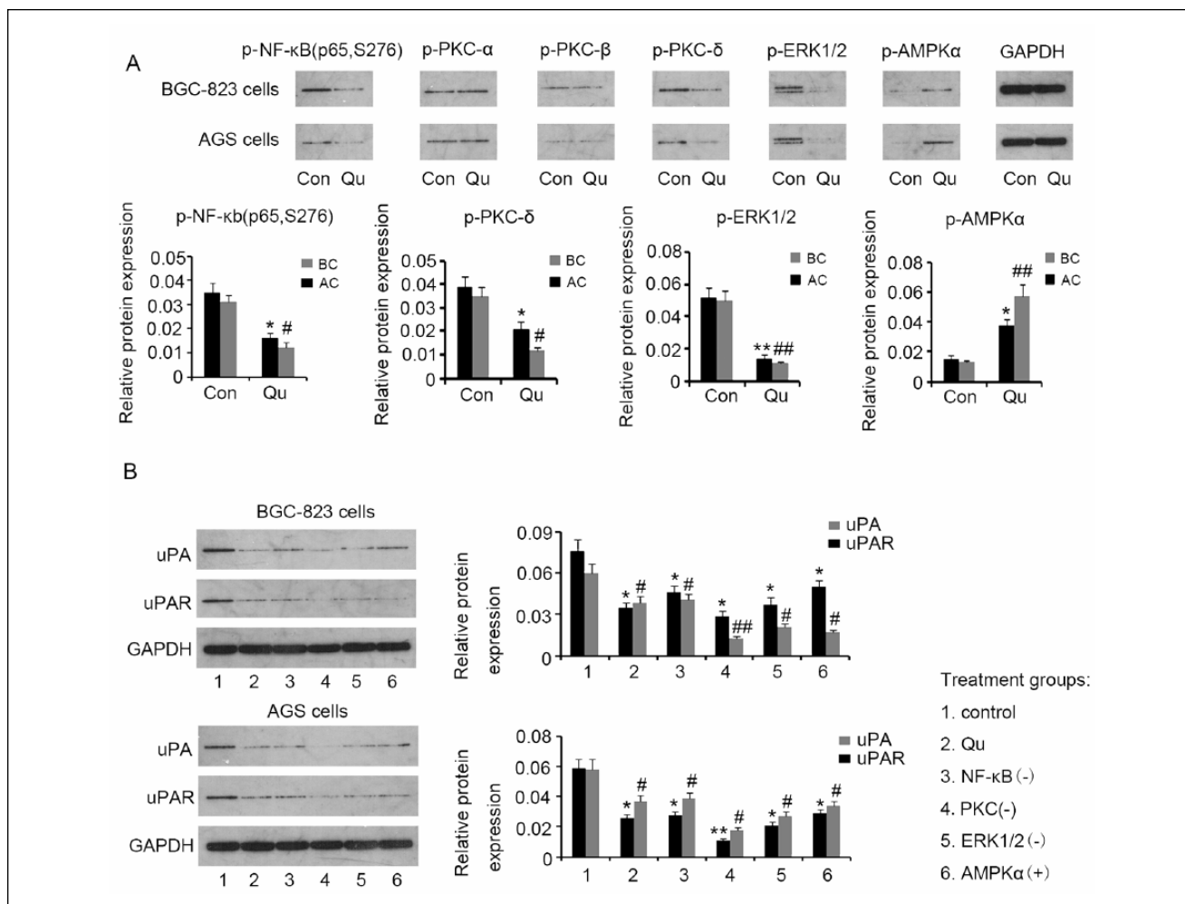
Figure 6. Suppression of the uPA/uPAR system by Qu may be mediated by NF-κb, PKC-δ, ERK1/2, and AMPKα. (A) Phosphorylation levels of NF-κb (p65), PKC-α, PKC-β, PKC-δ, ERK1/2, and AMPKα were evaluated in BGC823 and AGS cells by Western blotting, after treatment with 10 μM Qu for 72 hours. Qu treatment was associated with inhibition of NF-κb, PKC-δ, and ERK1/2 activities and with AMPKα activation. (B) Specific inhibitors of NF-κb (p65), PKC, and ERK1/2, as well as activators of AMPKα were used to assess their roles in uPA and uPAR regulation. BGC823 and AGS cells were incubated with 9 μM JSH-23, 10 nM Go6983, 12 μM SCH772984, or 4.5 μM A-769662 for 72 hours. Similar to Qu, specific inhibitors of NF-κb, PKC, and ERK1/2, and an AMPKα activator suppressed uPA and uPAR expression in GC cells. Bars representing the average of data from 3 independent tests. *P < .05, **P < .01, #P < .05, ###P < .01 versus control group. Qu, quercetin; uPA, urokinase plasminogen activator; uPAR, uPA receptor; GAPDH, glyceraldehyde-3-phosphate dehydrogenase; NF-κb, nuclear factor-κb; PKC, protein kinase C; ERK1/2, extracellular signal-regulated kinase 1/2; AMPKα, adenosine monophosphate activated protein kinase α; NF-κb(-), NF-κb inhibition with the inhibitor; PKC(-), PKC inhibition with the inhibitor; ERK1/2(-), ERK1/2 inhibition with the inhibitor; AMPKα(+), AMPKα activation with the activator.
