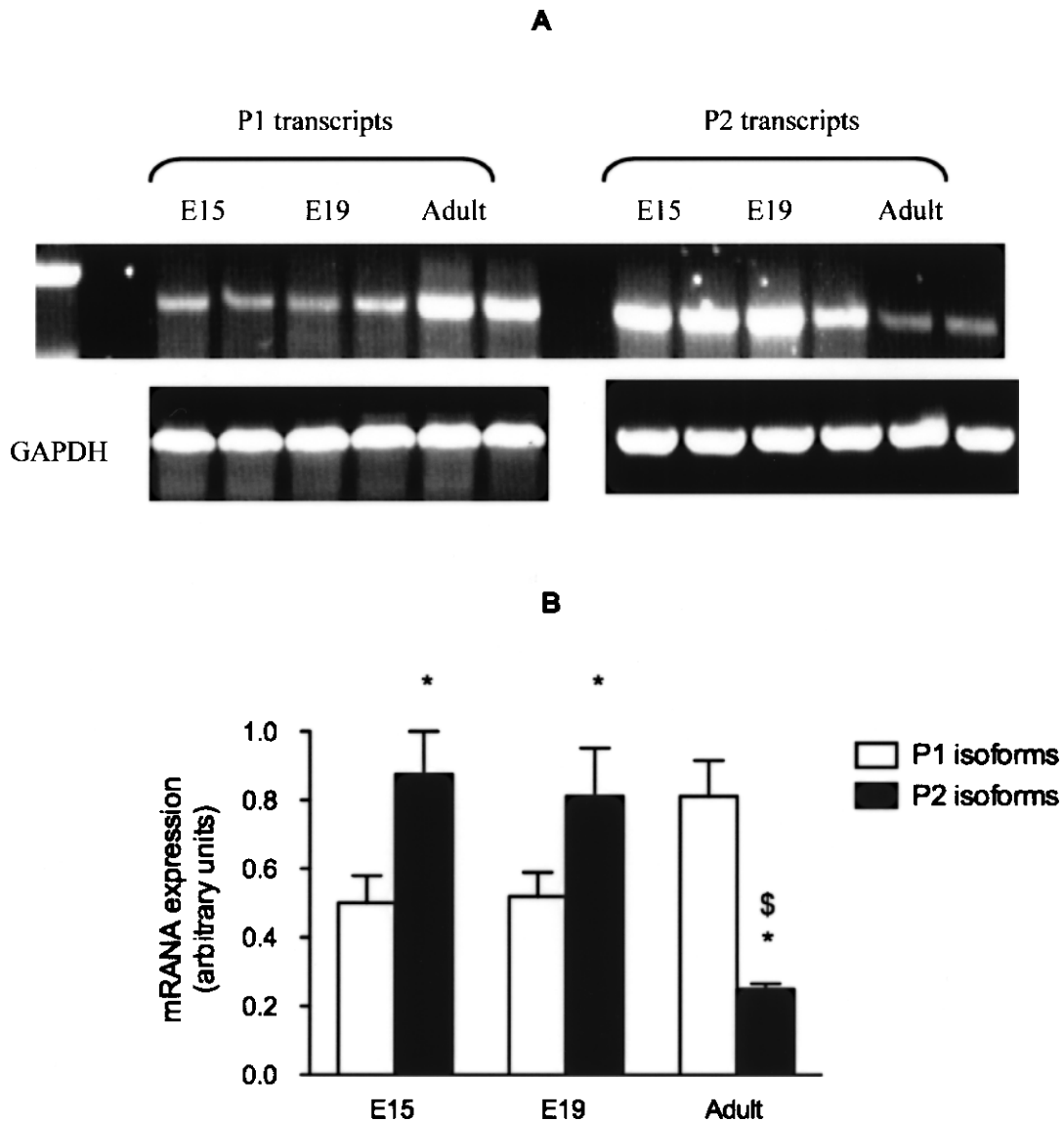
Figure 2. Expression of P1 and P2 HNF4- \alpha isoforms in mouse liver. HNF4- \alpha mRNA from mouse fetal (E15 and E19) and adult liver was measured by real-time RT-PCR using P1- or P2-specific primers. GAPDH was used as control housekeeping gene. (A) RT-PCR products separated on agarose gel and (B) relative mRNA content (mean \pm SEM) in the liver at different ages. * p < 0.05 versus P1; $ p < 0.05 versus fetal (E15, E19).
