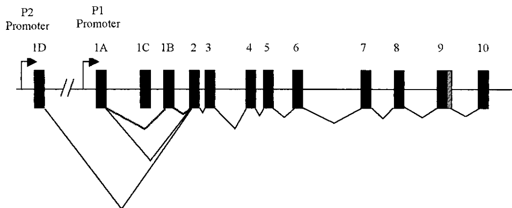
Figure 1. Systematic representation of the HNF4- \alpha gene structure. Exons are shown as boxes. The arrows represent the two alternative promoters and the lines linking exons indicate splicing events.
