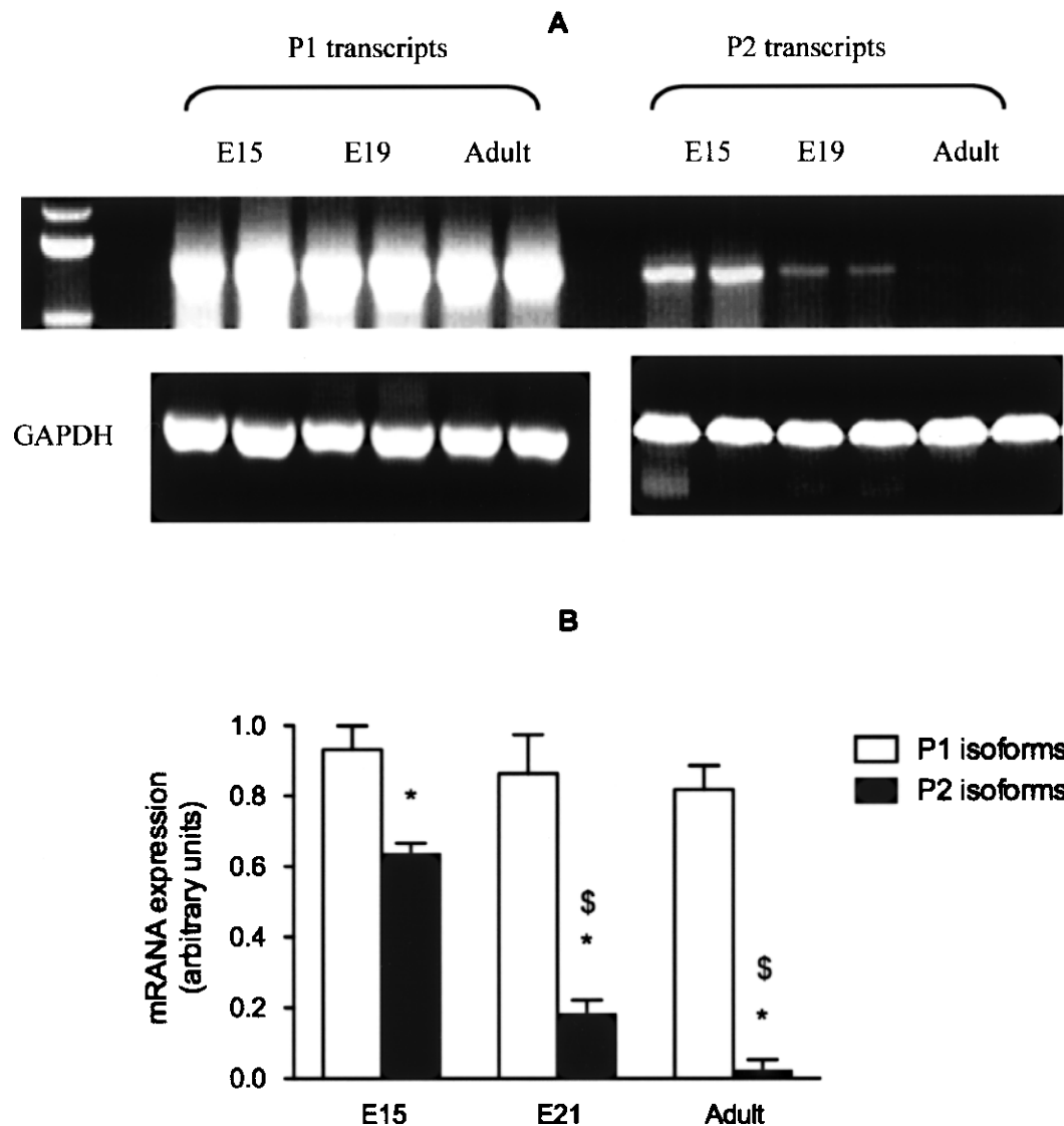
Figure 3. Expression of P1 and P2 HNF4- \alpha isoforms in rat liver. HNF4- \alpha mRNA from rat fetal (E15 and E21) and adult liver was measured by real-time RT-PCR using P1- or P2-specific primers. GAPDH was used as control housekeeping gene. (A) PCR products separated on agarose gel and (B) relative mRNA content (mean \pm SEM) in the liver at different ages. * p < 0.05 versus P2; $ p < 0.05 versus E15.
