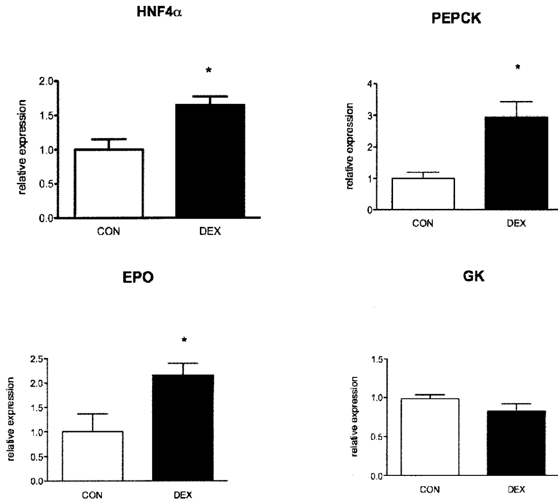
Figure 5. Effect of dexamethasone on HNF4- \alpha and its target genes. Hepatic expression of HNF4- \alpha , PEPCK, EPO, and glucokinase (GK) mRNA was measured in E21 fetuses of dams that received dexamethasone (DEX) or vehicle (CON) during the last week of pregnancy. Results (mean \pm SEM) represent mRNA levels relative to control animals ( n = 8 per group). * p < 0.05 versus control.
