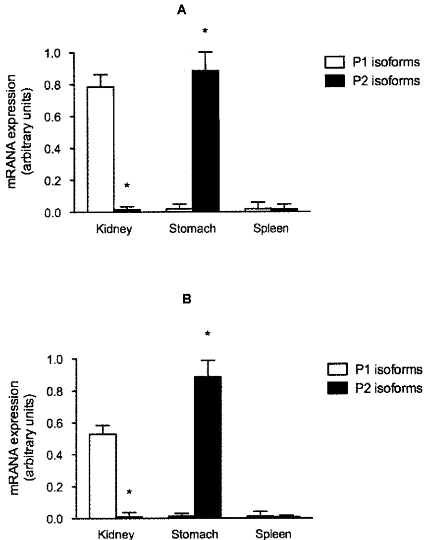
Figure 4. Expression of P1 and P2 HNF4- \alpha isoforms in kidney, stomach, and spleen. HNF4- \alpha mRNA isolated from adult mouse (A) and rat (B) kidney, stomach, or spleen was analyzed by real-time RT-PCR using P1- or P2-specific primers. GAPDH was used as control housekeeping gene. * p < 0.05 P1 versus P2.
