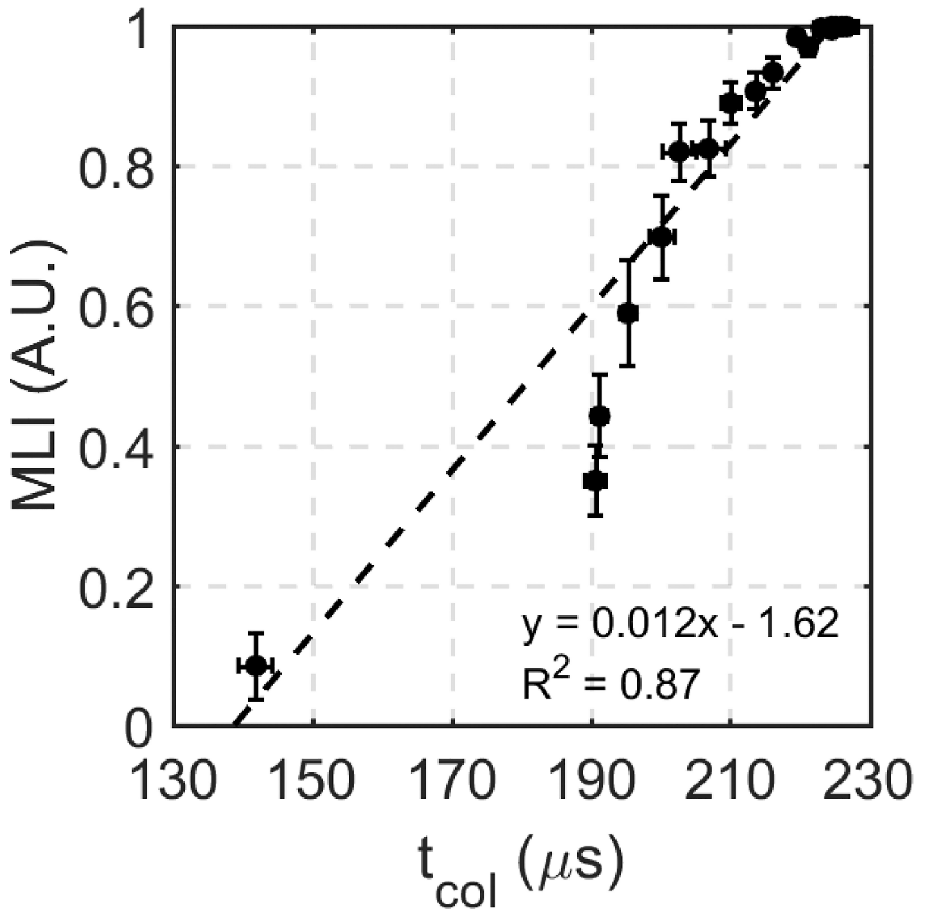
Figure 10. Linear correlation between t_{col} and MLI for 100 histotripsy pulses ( n=6 ).
