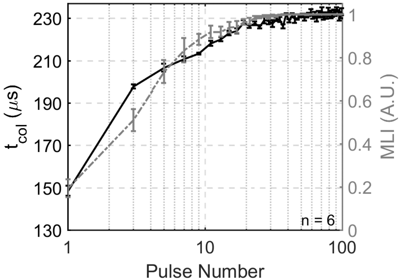
Figure 9. t_{col} (left y-axis) and MLI (right y-axis) vs. pulse number throughout 100 pulses. The majority of changes in t_{col} and MLI occur early in treatment and at the same time. The change in t_{col} is greater than the change in MLI in the first several pulses, but both metrics even out quickly and reach a plateau threshold around 40 pulses.
