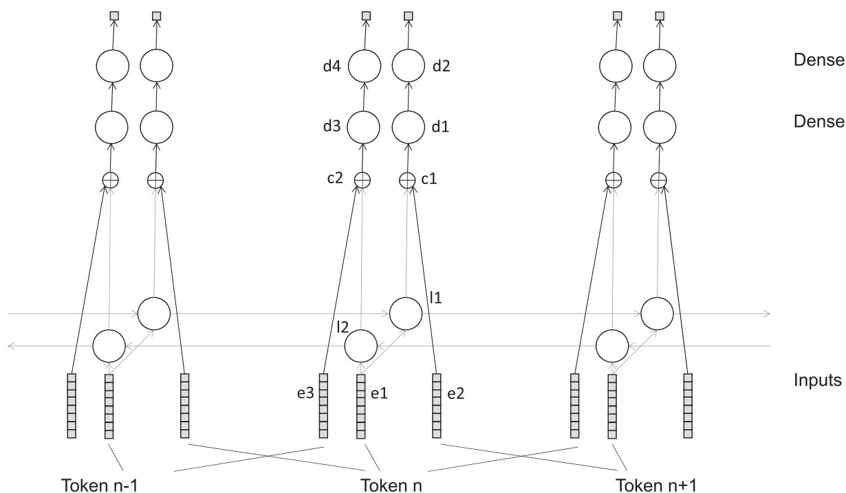
Figure 1. Pre-training network.
