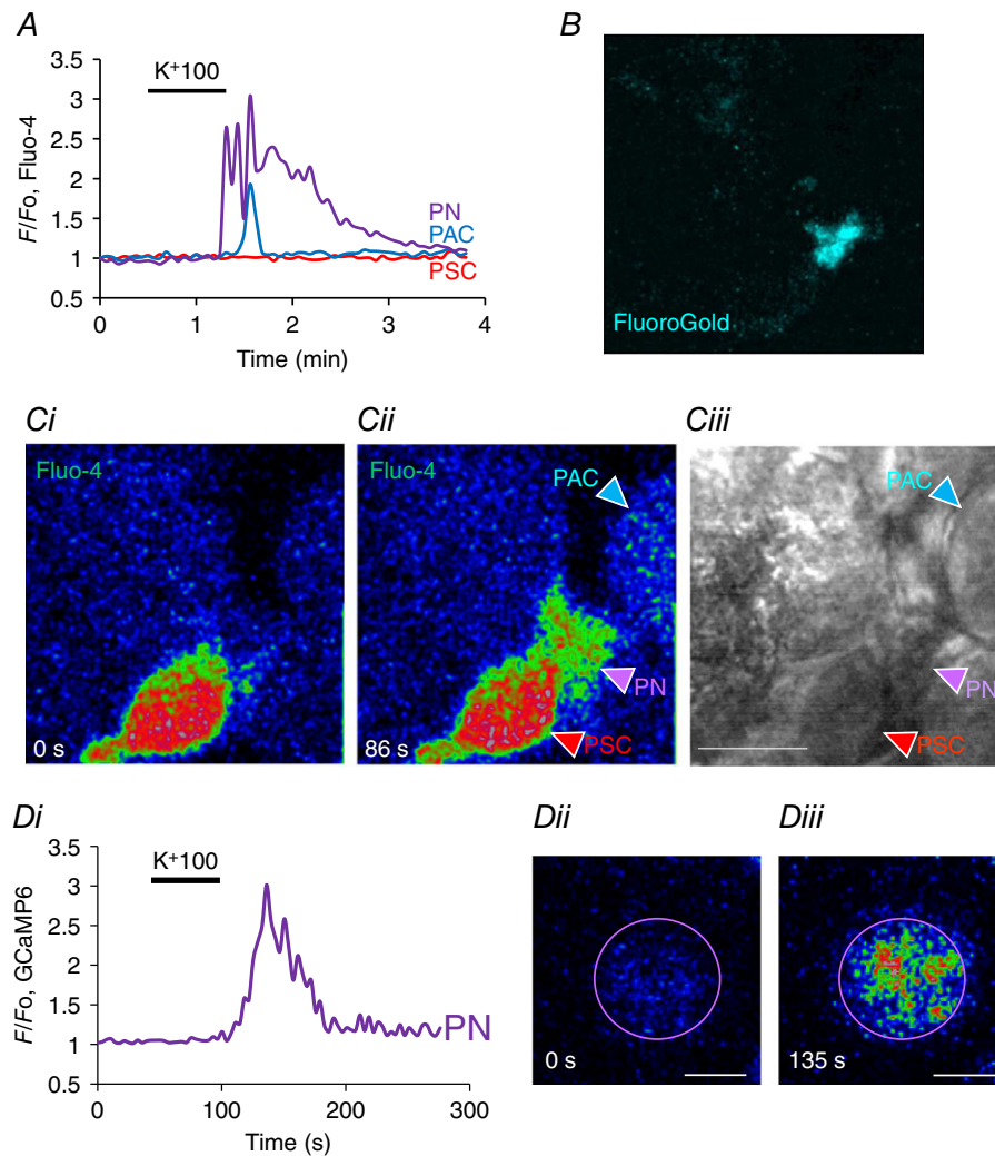
Figure 3. \text{K}^+ depolarization evokes \text{Ca}^{2+} signals in labelled pancreatic neurons
