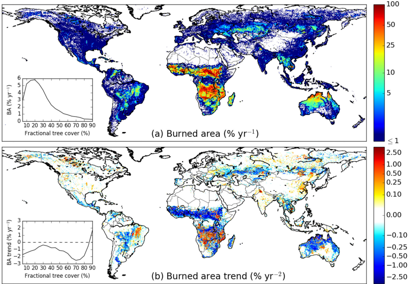
Fig. 1. Satellite observations of (a) mean annual burned area and (b) trends in burned area (GFED4s, 1998 - 2015) show a decline of fire activity across the world's tropical and temperate grassland ecosystems and land use frontiers in the Americas and Southeast Asia. Line plots (inset) indicate global burned area and trend distributions by fractional tree cover (28).
