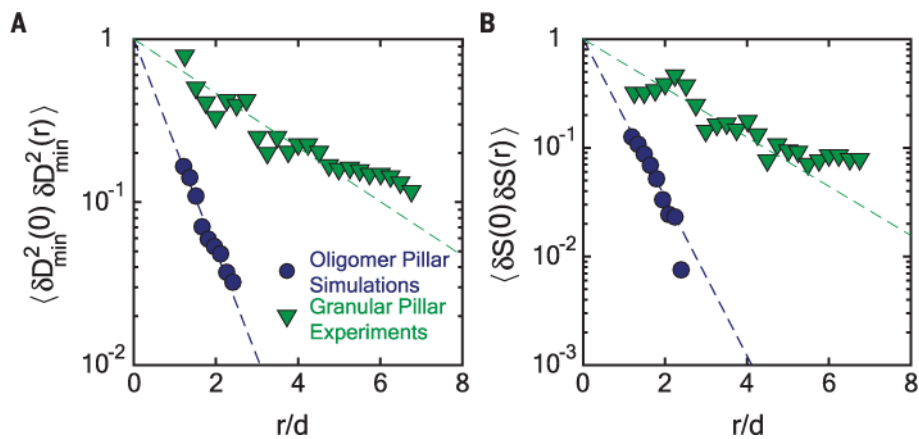
Fig. 1. Spatial correlations in D_{\min}^2 and softness fields
