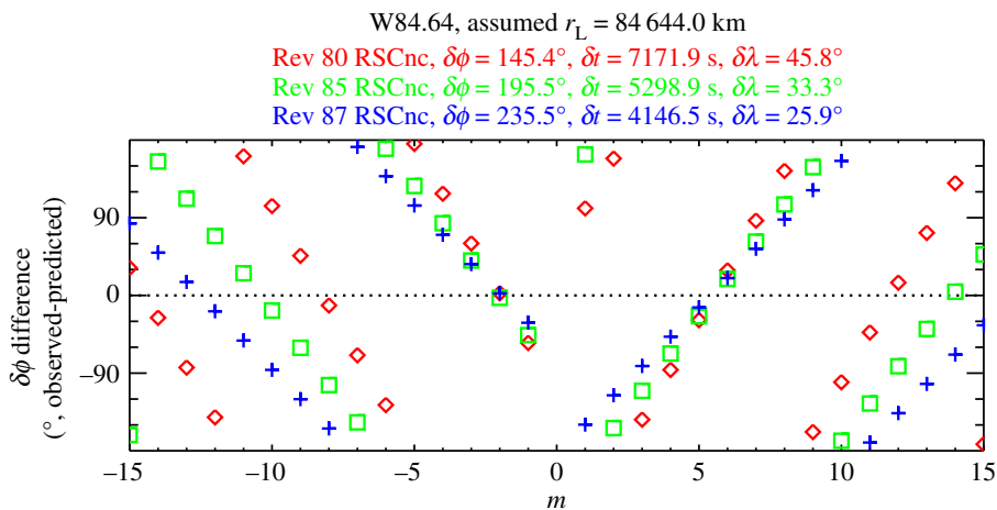
Figure 21. Plot showing the difference between the observed and predicted values of \delta\phi between the ingress and egress cuts of the RS Cancri occultations for the wave W84.64 as a function of the assumed m -number. Note that the residuals for all three observations are close to zero when m = -2, +5 and +6 , so these values of m are the ones most consistent with the observed phase differences. Figure from Hedman & Nicholson [4].
