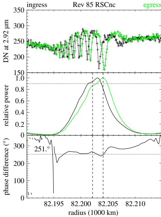
Figure 18. Results of the wavelet calculations of the phase difference in wave W82.21 between the ingress and egress cuts from the Rev 85 RS Cancri occultation. The top panel shows two occultation profiles, while the middle panel shows the integrated wave power E_{\text{eff}}(r) between wavenumbers of 2\pi/(5 \text{ km}) and 2\pi/(0.1 \text{ km}) . The bottom panel shows the phase difference \delta\phi(r) = \phi_{\text{egress}}(r) - \phi_{\text{ingress}}(r) between these two cuts (see text for explanations of the dashed and dotted lines). Note that the average phase difference is computed using only the data where the average E_{\text{eff}} of the two profiles is above 0.9. The average phase difference is near 240^\circ , which is consistent with the offset between the ingress and egress wave profiles noted in figure 16. Figure from Hedman & Nicholson [4].
