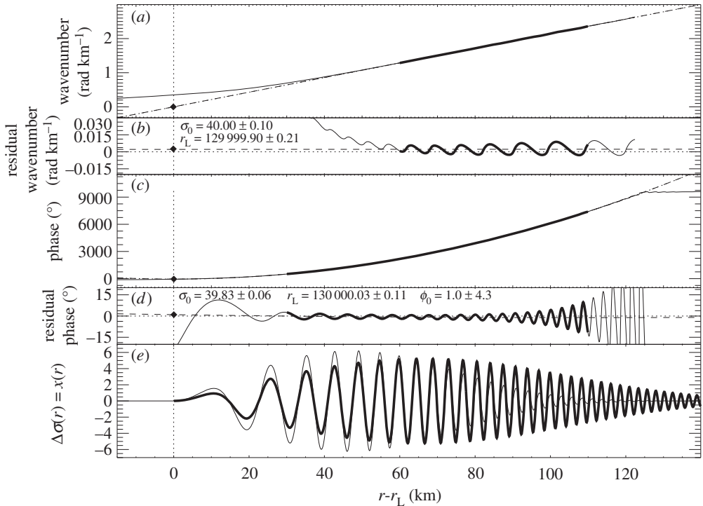
Figure 3. (a) Calculated wavelet ridge (§3g), as in figure 2c (solid line); the expected wavenumber k_{DW}(r) (dotted line). The region of the wavelet ridge plotted in bold was used in a linear fit (dashed line); the y = 0 point is plotted as a solid diamond. (b) All three curves from figure 3a, shown as residuals with the expected wavenumber k_{DW}(r) . (c) Calculated wavelet phase \bar{\phi}_W(r) , as in figure 2b, ‘unwrapped’ to show how phase accumulates quadratically (solid line); the expected phase \phi_{DW}(r) (dotted line). The region of \bar{\phi}_W(r) shown in bold was used in a quadratic fit (dashed line); the zero-derivative point is plotted as a solid diamond. (d) All three curves from figure 3c, shown as residuals with the expected phase \phi_{DW}(r) . (e) The input synthetic density wave from figure 2a (solid line); the fitted density wave, after the analysis of §4a(i), but still with randomly chosen values of \xi_D and A_L (bold solid line). Fitted values given in the figure can be compared with the input parameters (table 1) used to generate the wave. Figure from Tiscareno et al. [11].
