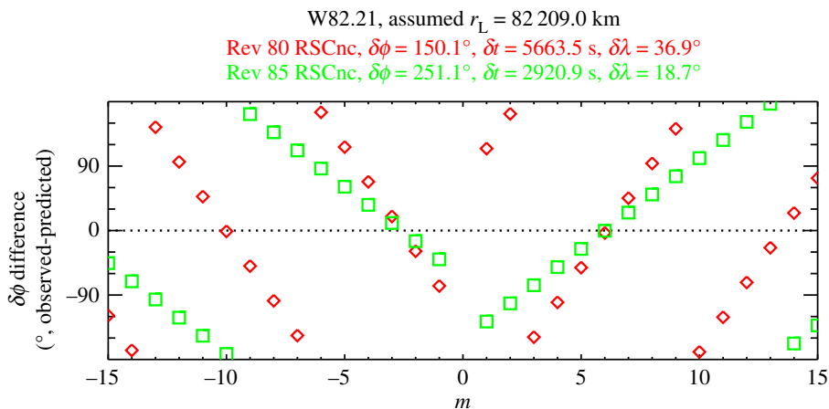
Figure 20. Plot showing the difference between the observed and predicted values of \delta\phi between the ingress and egress cuts of the RS Cancri occultations for the wave W82.21 as a function of the assumed m -number, given the stipulated \delta\lambda and \delta t values. Different symbols correspond to different pairs of occultation cuts. Note that the residuals for both observations are close to zero when m = -2, -3 and +6 , so these values of m are the ones most consistent with the observed phase differences. Figure from Hedman & Nicholson [4].
