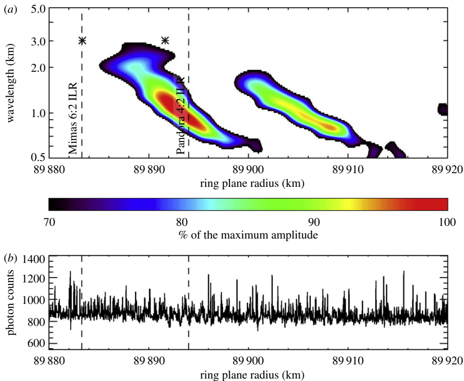
Figure 14. (a) Wavelet power profile of the Mimas 6:2 and Pandora 4:2 SDWs in the C ring, derived by co-adding wavelet profiles from UVIS occultations via the WWZ process. The y -axis is wavelength, rather than wavenumber as in other figures in this work. (b) One of the individual UVIS occultations from which the wavelet profile in a was computed, namely \beta Centauri from Rev 85. The waves are not visible by eye in this profile. Figure from Baillié et al. [22].
