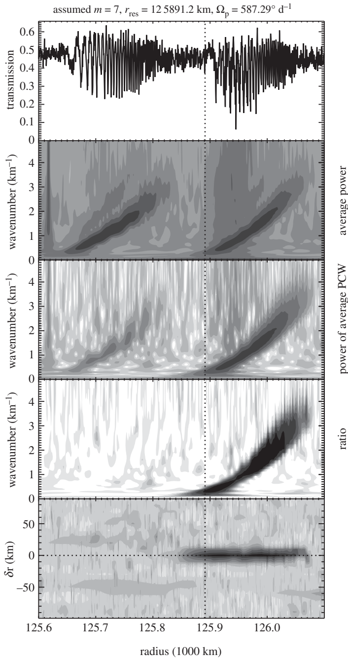
Figure 24. Sample analysis of the Prometheus 7:6 wave in the A ring as a function of radius from the Rev 89 occultation by \gamma Crucis. The two density waves clearly visible in this profile are due to the Pandora 6:5 and Prometheus 7:6 resonances. The second panel shows the average wavelet power \bar{E} for the \gamma Crucis occultations, with clear diagonal bands associated with both waves. The third panel shows the power of the average phase-corrected wavelet E_\phi , assuming m = 7 and a pattern speed appropriate for the Prometheus 7:6 resonance (the exact resonance location is marked by the vertical dotted line). Note that this highlights the right-hand wave. The fourth panel shows the ratio of the above powers \mathcal{R} , and shows only the signal from that wave. Finally, the bottom panel shows the peak value of \mathcal{R} as a function of radius and assumed pattern speed, parametrized as a displacement \delta r from the expected Prometheus 7:6 resonance location (marked with a horizontal dotted line). Note that the maps of \bar{E} and E_\phi use a common logarithmic stretch, while the maps of \mathcal{R} use a linear stretch. Figure from Hedman & Nicholson [24].
