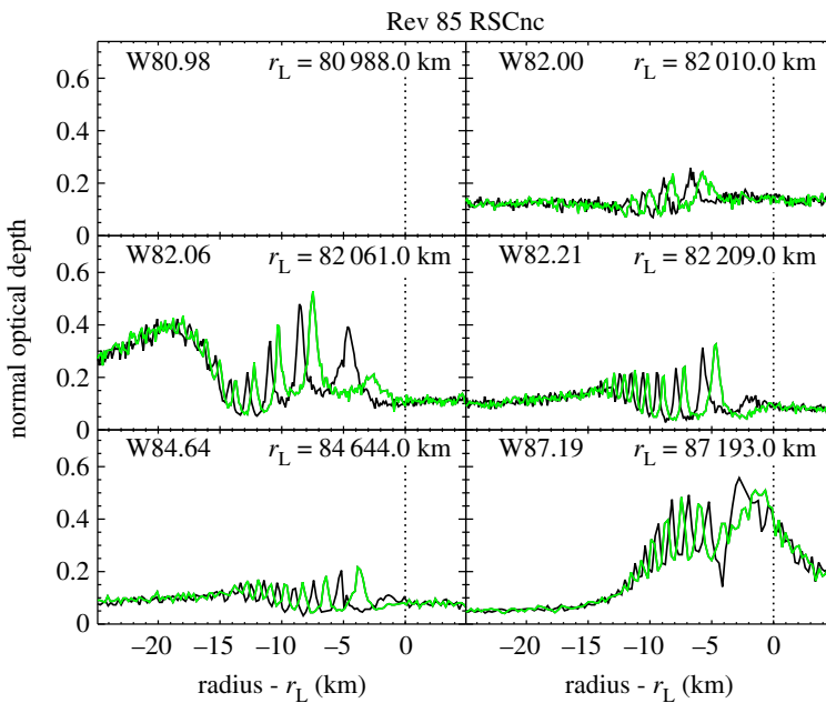
Figure 16. Profiles of six waves in the C ring obtained during the occultation of the star RS Cancri on Rev 85. The black profiles were obtained during ingress, while the green profiles were obtained during egress. Note that the phase differences between the waves seen in ingress and egress are again the same for the three waves found around 82 000 km. This implies that all these waves have the same m -numbers. The two waves found outside 84 000 km also show similar phase differences, indicating that they may have the same m -number as each other. Figure from Hedman & Nicholson [4].
