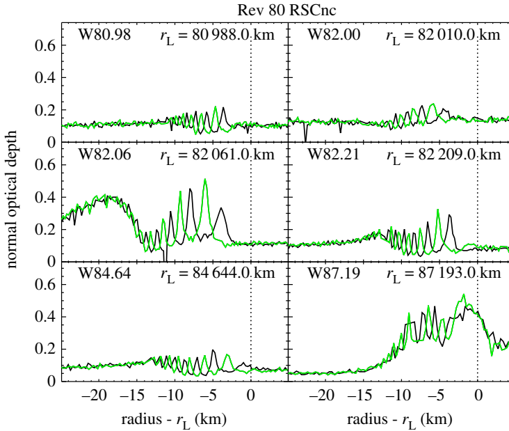
Figure 15. Profiles of six waves in the C ring obtained during the occultation of the star RS Cancri on Rev 80. The black profiles were obtained during ingress, while the green profiles were obtained during egress. The normal optical depth values assume the star's elevation angle above the rings is 29.96^\circ . Note that the phase differences between the waves seen in ingress and egress are the same for the three waves found around 82 000 km. This suggests that all these waves have the same m -numbers. Figure from Hedman & Nicholson [4].
