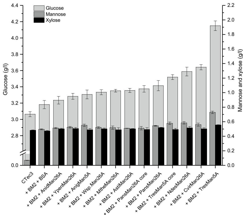
Fig. 3 Softwood saccharification. Endomannanases or BSA were added in equal molar amounts on top of Cellic ® CTec3 plus an A. niger GH2 \beta -mannosidase (BM2). Samples were taken after 24 h saccharification at 30 °C. Glucose (g/l, light grey), mannose (dark grey) and xylose (black) yields are given as mean values \pm SD ( n = 3 ). One-way ANOVA analyses can be seen in Additional file 1: Table S3. Yields from 48 and 144 h can be seen in Additional file 1: Figure S2
