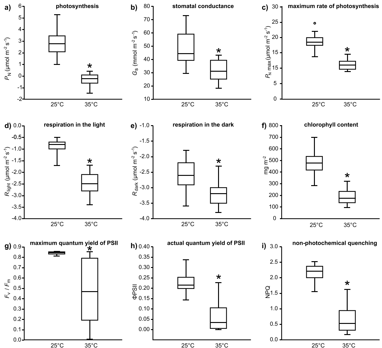
Figure 4. Box plots representing the effects of growth at 25 and 35°C on the physiology of Ginkgo biloba leaves: (a) photosynthesis (one-way ANOVA F_{1,53} = 157.6 ; P = 1.7 \times 10^{-17} ); (b) stomatal conductance (one-way ANOVA F_{1,53} = 31.3 ; P = 7.9 \times 10^{-7} ); (c) maximum rate of photosynthesis (one-way ANOVA F_{1,53} = 181.2 ; P = 9.8 \times 10^{-19} ); (d) respiration in the light (one-way ANOVA F_{1,53} = 261.1 ; P = 4.0 \times 10^{-22} ); (e) respiration in the dark (one-way ANOVA F_{1,53} = 30.1 ; P = 1.2 \times 10^{-6} ); (f) foliar content of chlorophyll a and b (one-way ANOVA F_{1,53} = 150.1 ; P = 4.3 \times 10^{-17} ); (g) maximum quantum yield of PSII (one-way ANOVA F_{1,53} = 52.6 ; P = 1.8 \times 10^{-9} ); (h) actual quantum yield of PSII (one-way ANOVA F_{1,53} = 106.08 ; P = 3.0 \times 10^{-14} ), and; (i) non-photochemical quenching (one-way ANOVA F_{1,53} = 250.4 ; P = 1.0 \times 10^{-23} ). Box plots presented as in Fig. 1.
