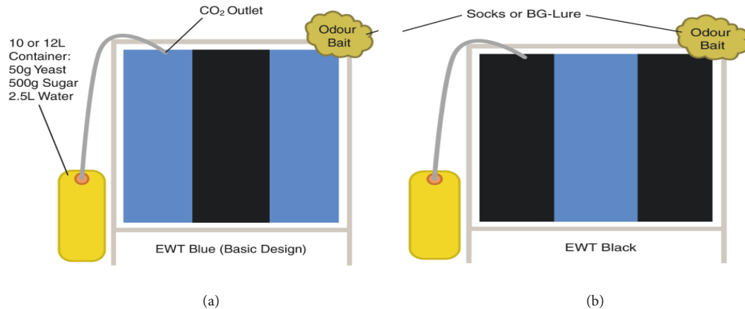
FIGURE 5: Blue and black trap designs showing position of CO 2 and odour baits. Blue screens with a black vertical stripe (basic design) were used for all trapping experiments in Uganda. Black screens with a blue vertical stripes were additionally used in Tanzania (source: Hendy et al. , 2017).
