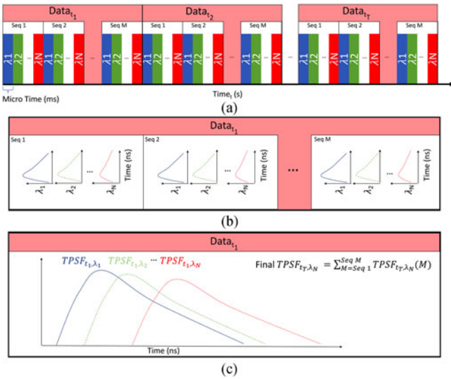
Fig. 2. Diagram of the acquisition sequence. (a) Diagram of the timing of the acquisition sequence. The TPSF at each wavelength is acquired sequentially with a small integration time per wavelength (10th of microseconds). Then this sequence is repeated M times. This operation is repeated for each time point. (b) Example of the acquisition of the TPSF for the first time point. This illustrates the sequential acquisition of the TPSF for each wavelength. (c) Final TPSF for the first time point. All the TPSFs of every sequence within the first time point are summed up at each wavelength and saved in the same file.
