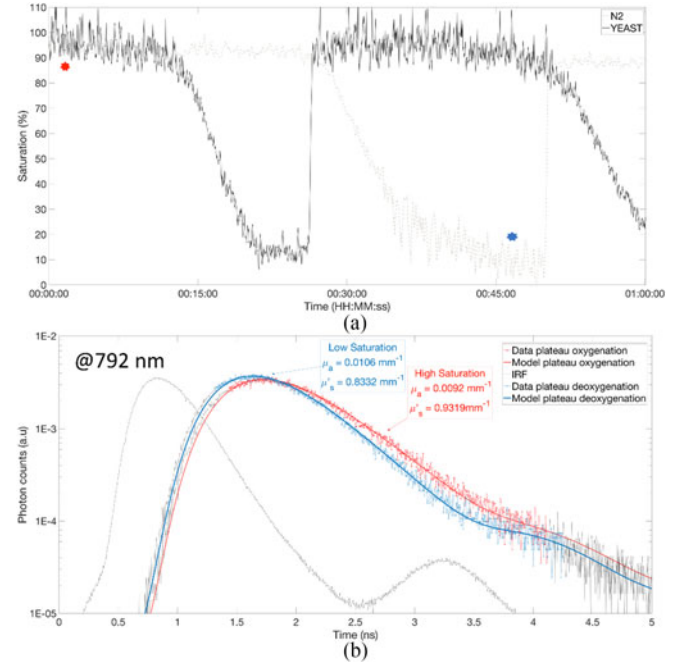
Fig. 11. (a) evolution of the saturation of the yeast (solid black) and N 2 (dashed grey) phantoms over the first hour of the experiment. (b) Example of the fitting of the optical properties for the N 2 phantom at 792 nm. The blue curve represents a low saturation point and the red curve represents a high saturation point. The exact timing of those points is reported with stars on part (a).
