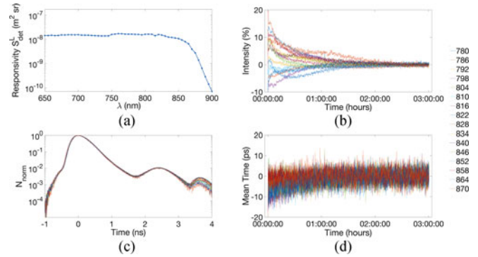
Fig. 7. Summary of the basic characteristics of the system. (a) Responsivity of detector 2 (b) Stability of the intensity of the IRF for 16 wavelengths. Intensity expressed as the percentage of variation regarding the mean value of the last 30 minutes. (c) IRF of 16 wavelengths of detector 2 (d) Stability of the mean time of flight of the IRF for 16 wavelengths. Mean time expressed as the mean time of flight variation regarding the mean value of the last 30 minutes.
