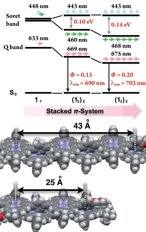
Fig. 3 Energy diagrams of the double-strands (1_n)_2 , and their geometry-optimized structures calculated using the MM + force field (HyperChem Ver. 8.0 software). The alkoxy side chains are omitted for visual clarity. The wavelengths denote the absorption maxima.
