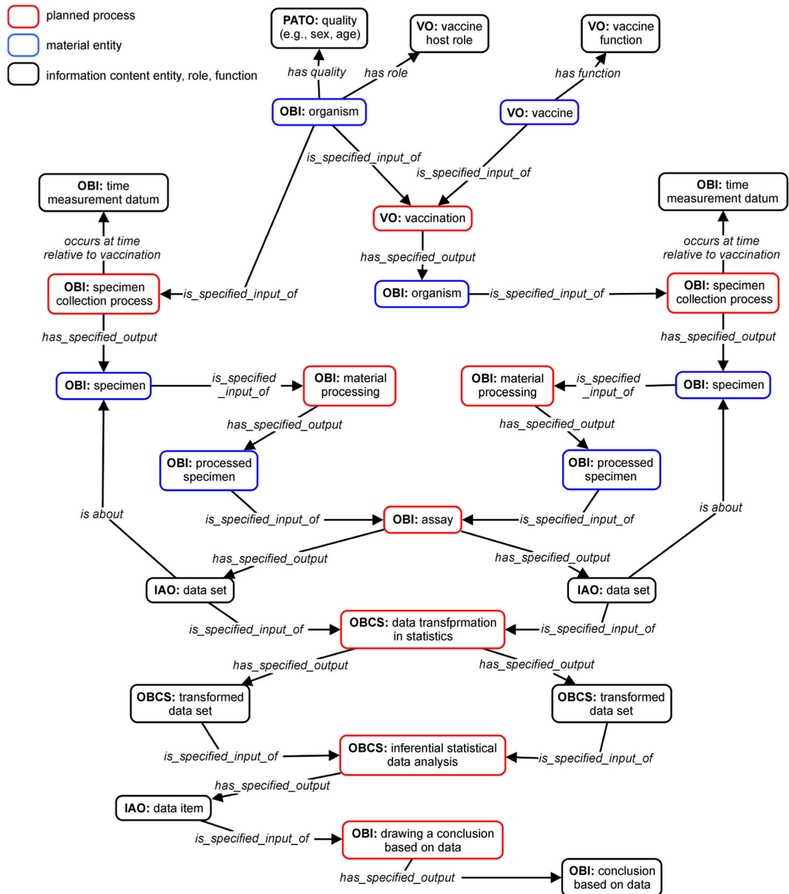
Figure 1. General modeling of vaccine immune response study and data analysis using VO and OBSC
