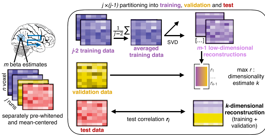
Fig. 3. Illustration of the combination of SVD and cross-validation, corresponding to step 2 in Fig. 2. For each searchlight or ROI, j (number of runs) n (number of voxels) \times m (number of beta estimates) matrices are used to estimate the functional dimensionality. For all possible partitions of j runs into training, validation and test data, we first average all training runs and build all possible low-dimensional reconstructions of these averaged data using SVD. All reconstructions are then correlated with the validation run, resulting in j - 1 correlation coefficients and respective dimensionalities. The dimensionality that results in the highest average correlation across j - 1 runs is picked as dimensionality estimate k for this fold and a k -dimensional reconstruction of the average of the training and validation runs is correlated with a held-out test-run, resulting in a final reconstruction correlation. In total, j reconstruction correlations are returned that can be averaged and tested for significance across participants using one-sample t-tests or alike. To derive a better estimate of the underlying dimensionality, the j dimensionality estimates per participant can be submitted to the hierarchical Bayesian model (step 4 in Fig. 2).
