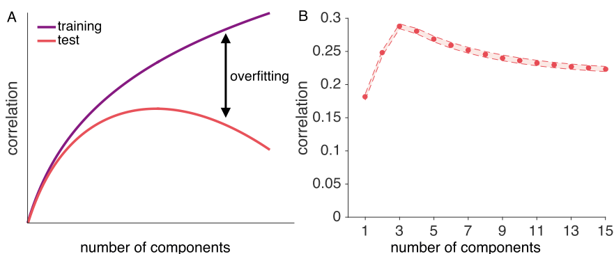
Fig. 1. Illustration of the concept of overfitting and generalizability. A: As more components are added to a low-dimensional reconstruction, the correlation between the training data and the reconstruction approaches the maximum of 1 for a full-dimensional reconstruction (purple curve). Adding components is equivalent to adding model parameters to improve fit, which reduces the model’s bias and increases its variance. For the correlation between the reconstructed training and independent test data (red curve), adding components initially improves performance but at some point reduces performance due to overfit (see Parpart et al., 2018, for a related illustration). B: Reconstruction correlations achieved by all possible low-dimensional reconstructions for a simulated ground-truth dimensionality of 4. Reconstruction correlations rise as more components are added up to the point where the true dimensionality is reached, and decrease afterwards. Results are averaged across 6 runs and 1000 simulated voxel patterns.
