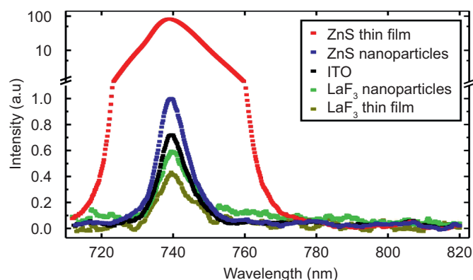
Figure 2 SHG signals obtained, with a fixed pump wavelength of 1480 nm and constant pump intensity, from a thin film of ZnS (red), a ZnS nanoparticle array (blue), a LaF 3 nanoparticle array (green), and a thin film of LaF 3 (dark yellow). All nanoparticle arrays and thin films were deposited on a glass substrate covered with a thin layer of ITO. The SHG signal from the ITO-covered substrate surface is shown in black.
