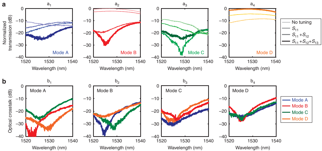
Figure 4 (a) Mesh configuration makes the transmission of the mode reconstructed at port Out 1 progressively increase a 4 , while the crosstalk due to the concurrent modes A a 1 , B a 2 and C a 3 reduces. (b) Reconstruction of mode A b 1 , mode B b 2 , mode C b 3 , and mode D b 4 at port Out 1 can be achieved with less than -20 dB residual crosstalk of the three concurrent modes over a bandwidth of ~10 nm.
