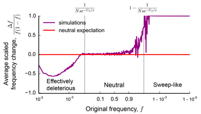
Figure 8 The average change in frequency of an allele observed at frequency f in an earlier sample. The pairs of frequencies were sampled in two consecutive sampling steps in Wright–Fisher simulations in which N = 10^5 , NU_d = 4Ns = 2 \cdot 10^4 . In the first step, the frequencies of all polymorphisms in the population and their unique identifiers were recorded. In the second sample, which was taken \delta t = Ne^{-U_d/s} generations later, the frequencies of all polymorphisms seen in the first sample were recorded [if a polymorphism had gone extinct, or fixed, a frequency f(\delta t) = 0 , or 1, was recorded]. The average represents the average frequency change over many distinct polymorphisms and the curve has been smoothed using a Gaussian kernel with width < 5\% of the minor allele frequency.
