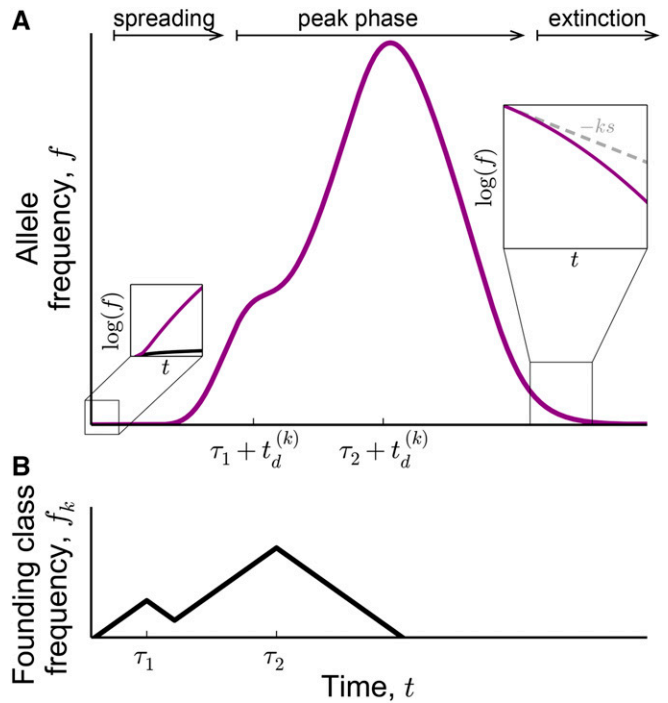
Figure 6 Schematic of (A) the trajectory of the total allele frequency, and (B) the trajectory of the frequency of the portion of the allele that remains in the founding class. Soon after arising in the founding class, the allele frequency rapidly increases in the spreading phase of the trajectory. Early in this phase, the total allele frequency (purple) becomes much larger than the frequency of the founding genotype [black line in left inset of (A)]. In the peak phase of the trajectory, the total allele frequency trajectory represents a smoothed-out and amplified version of the trajectory in the founding class [the relationship between the total allele frequency (purple curve) and the founding genotype frequency (black curve) is based on Equation 22]. In the extinction phase of the trajectory, the allele frequency declines at an increasing rate [right inset of (A)]. We describe the extinction phase in more detail in Appendix E and in the section of the main text titled The trajectories of high frequency alleles , 1 - f \ll 1 , where we also explain how the rate of extinction changes with the frequency.
