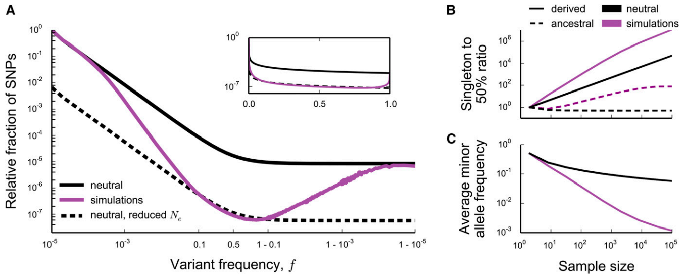
Figure 1 (A) The (unfolded) average site frequency spectrum of neutral alleles along a nonrecombining genomic segment experiencing strong background selection deviates strongly from the prediction of neutral theory. The purple line shows the simulated neutral site frequency spectrum in Wright–Fisher simulations of an asexual population of N = 10^5 individuals, where deleterious mutations occur at rate NU_d = 5000 and all have the same effect on fitness Ns = 1000 . The black lines show the neutral expectation for the site frequency spectrum of a population of N and N_e = Ne^{-U_d/s} individuals (solid and dashed line, respectively). The inset shows the same data, but with the x -axis linearly scaled to emphasize intermediate frequencies. Simulated site frequency spectra were obtained by measuring whole-population neutral site frequency spectra in 10^5 Wright–Fisher simulations, in which neutral mutations were set to occur at rate NU_n = 10^3 , and by averaging and then smoothing the obtained curve using a box kernel smoother of width much smaller than the scale on which the site frequency spectrum varies (the kernel width was set to < 10\% of the minor allele frequency). (B and C) Statistics of the simulated site frequency spectrum (purple) can deviate from predictions of neutral theory (black) by many orders of magnitude in large samples, even though the effect of background selection will be small in small samples. (B) The average ratio of the number polymorphisms present as derived singletons (solid lines) or ancestral singletons (dotted lines) in the sample to the number present at 50% frequency, and (C) the average minor allele frequency of the sampled alleles.
