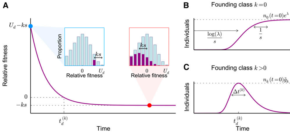
Figure 4 (A) The average fitness of a lineage comprising individuals carrying k deleterious mutations at time t = 0 (blue dot and blue inset). As the descendants of these individuals accumulate further deleterious mutations, the fitness of the lineage declines until the individuals accumulate an average of \lambda deleterious mutations (red dot) and reach their own mutation–selection balance, which is a steady-state Poisson profile with mean \lambda that has been shifted by the initial deleterious load, -ks , (red inset). (B) In the absence of genetic drift, the size of the lineage will increase at a rate proportional to its relative fitness. Lineages arising in the class with k = 0 deleterious
