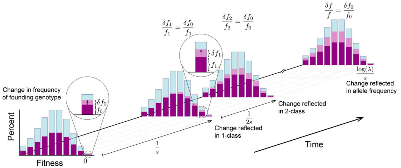
Figure 5 A schematic showing how a change in the frequency of the lineage in the mutation-free class propagates to affect the frequency in all classes of lower fitness. At time t = 0 , the lineage is in mutation–selection balance at total frequency f , when the frequency of the portion of the lineage in the 0-class changes suddenly from f_0 to f_0 + \delta f_0 . This change is felt in the 1-class 1/s generations later and propagates to the 2-class yet another 1/(2s) generations later. The lineage reaches a new equilibrium about \log(\lambda)/s generations later, when the total allele frequency is proportional to (f_0 + \delta f_0)e^\lambda .
