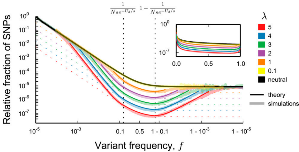
Figure 2 Comparison between the theoretical predictions for the site frequency spectrum and Wright-Fisher simulations. In all simulations, Nse^{-U_d/s} = 1000 \cdot e^{-5} \approx 6.73 , while the parameter \lambda = U_d/s varies from 5 to 0.1 (values shown on figure). Dashed lines show the expectations for a neutral population at reduced effective population size N_e = Ne^{-\lambda} . At frequencies smaller than 1/(N\sigma) (where \sigma = \sqrt{U_d s} ) and larger than 1 - 1/(N\sigma) , the theoretical predictions agree with the predictions for a neutral population with census size N (black line). Within the range 1/(N\sigma) < f < 1 - 1/(N\sigma) , the theoretical predictions (Equation 2) are given by colored lines. A single theory curve was constructed from Equation 2 by joining the piecewise forms using sigmoid func-
