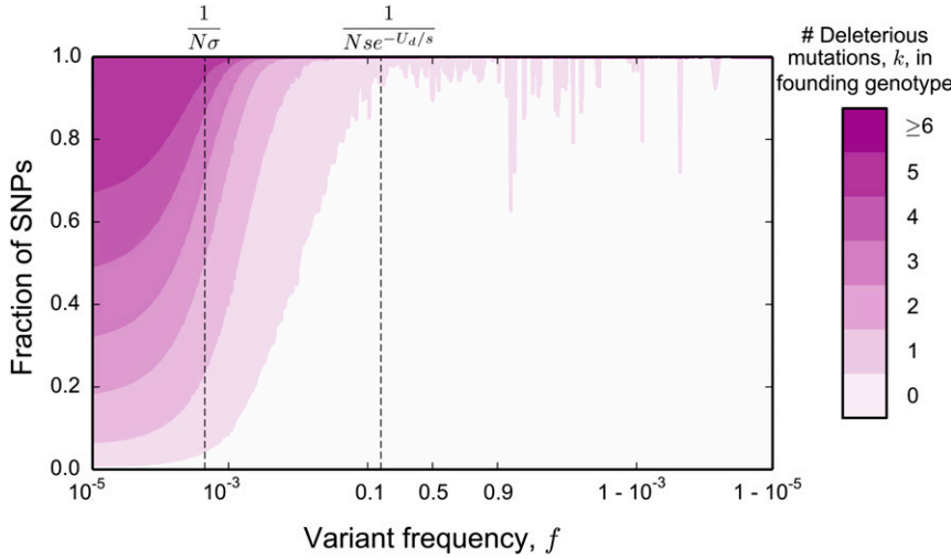
Figure 7 Proportions of polymorphisms at a given frequency that arose in genotypes that had a specified number of additional deleterious mutations compared to the most-fit genotype at the locus at the time they arose. The parameters in these simulations are the same as the parameters used to generate site frequency spectra in Figure 1 and Figure 3. Note that for frequencies f > 1/(Nse^{-\lambda}) , the entire site frequency spectrum comprises lineages that arose due to neutral mutations in the k = 0 class (with only a few exceptions that arise due to rare ratchet events).
