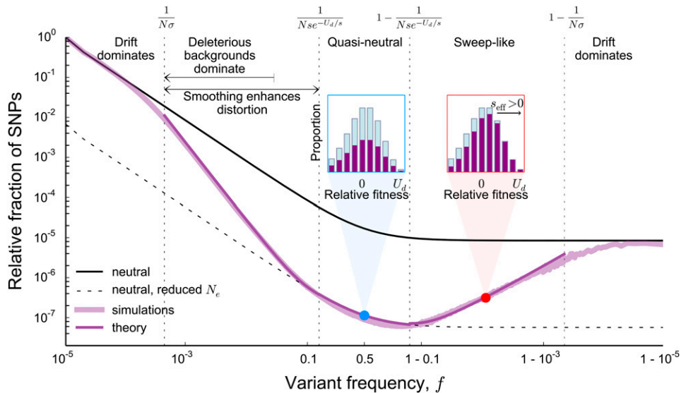
Figure 3 A summary of the dominant effects shaping the site frequency spectrum. The site frequency spectrum and theoretical predictions are reproduced from Figure 1 and Figure 2 ( \lambda = 5 ). At frequencies below 1/(N\sigma) and above 1 - 1/(N\sigma) , the allele frequency trajectories of the majority of neutral alleles are dominated by drift, resulting in neutral site frequency spectra corresponding to a population of size N . In contrast, linked selection has a crucial impact for 1/(N\sigma) < f < 1 - 1/(N\sigma) . The rapid falloff of the site frequency spectrum for 1/(N\sigma) < f < 1/(Nse^{-\lambda}) is primarily a result of allele frequency trajectories having fundamentally nonneutral properties. In this regime, the number of backgrounds on which neutral alleles can arise also declines with the frequency f . As we show later, for f \ll 1/(Nu_d e^{-\lambda}) , the site frequency spectrum is dominated by
