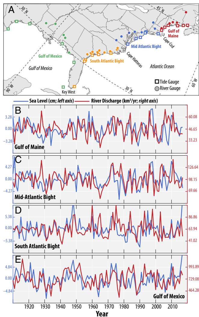
Fig. 1. Observations of coastal sea-level and river-discharge variations. (A) Locations of 26 river stations (circles) and 24 tide gauges (squares) on the Gulf of Maine (red), Mid-Atlantic Bight (blue), South Atlantic Bight (yellow), and Gulf of Mexico (green) used here. See SI Appendix, Tables S1–S3 for more details on the data sites. Subsequent panels show detrended annual water-year averages of integrated river discharge (red) and averaged sea level (blue) over the (B) Gulf of Maine, (C) Mid-Atlantic Bight, (D) South Atlantic Bight, and (E) Gulf of Mexico versus water year. Time series have been adjusted for large-scale climate modes as explained in the text and SI Appendix .
