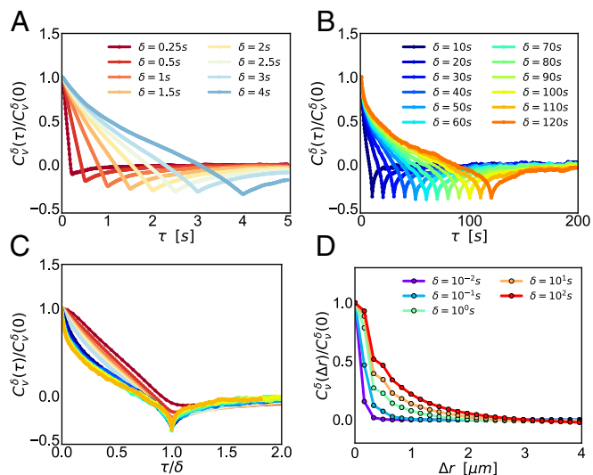
Fig. 3. Viscoelastic behavior in chromatin. (A and B) Velocity autocorrelation functions C_v^\delta(\tau) = \langle v(t+\tau) \cdot v(t) \rangle with v(t) = 1/\delta(r(t+\delta) - r(t)) obtained from the simulations for different time intervals \delta and plotted as a function of the time delay \tau . We see the chromosome behaves as a viscoelastic medium. The same viscoelastic behavior was observed in vivo by Lucas et al. (3) in mammalian cells. Curves for the shortest time scales, shown in A, deviate from exact self-similarity, with a deepening negative peak. This behavior, not seen in experiments, is an artifact of the Langevin dynamics integrator, whose damping time corresponds to 1 s and is therefore comparable to the shorter time scales tested. Curves corresponding to longer time intervals, shown in B, are instead markedly self-similar. The negative peak stabilizes at a value of -0.375 . Global confinement would give a value of -0.5 (25). Interestingly, the value -0.375 is quite similar to the experimentally determined value in ref. 3. (C) The simulated velocity autocorrelation functions measured for different time lags, when rescaled by their time lag \delta , collapse reasonably well to a single curve. Experimental data collapse in the same universal fashion (3). (D) Velocity correlations of the loci C_v^\delta(\Delta r) = \langle v(r_i(t), \delta) \cdot v(r_j(t), \delta) \delta(|r_i(t) - r_j(t)| - \Delta r) \rangle as a function of the scalar distance in space between the loci, \Delta r , and for different time lags \delta . Simulations show that spatial coherence increases when one increases the time lag in observations. Similar behavior was seen for correlations in HeLa cells in ref. 4. The coherence of motion in the simulated conformational ensembles increases monotonically over time lags \delta spanning four orders of magnitude. The size of the correlated region is predicted to be on the micrometer scale, once again comparing favorably with what is seen in the laboratory (4).
