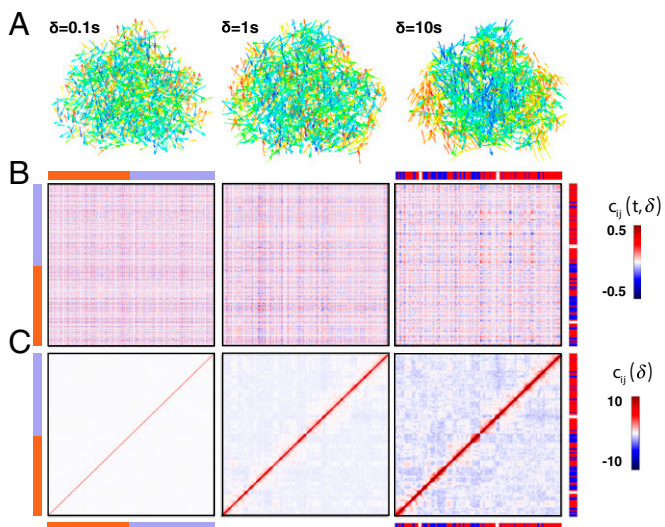
Fig. 4. Coherent motion in chromatin. (A) The 3D vector field of loci velocities v(r, t) = 1/\delta(r(t+\delta) - r(t)) for a typical configuration at time t . Velocities are measured over increasing time intervals \delta from left to right. The color of the arrows indicates the direction of the velocity vector, with red marking the outward-oriented z axis. It is visually evident that increasing the time interval increases the size of the regions of coherent motion. This result is qualitatively similar to what was observed in ref. 4. (B) Matrix of the instantaneous velocity correlations c_{ij}(t, \delta) = v(r_i(t), \delta) \cdot v(r_j(t), \delta) between loci i and j for a typical configuration at time t and for increasing time intervals \delta . The color of a pixel indicates the instantaneous velocity correlation increasing from blue to red. The sidebars indicate chromatin structural type annotations (type A in red and B in blue) and chromosome identity (chromosome 17 in orange and 18 in lavender). The regions of coherence increase in size as indicated by the coarsening of the plaid pattern when moving from left to right, as one increases the coarse-graining time interval \delta . (C) Ensemble-averaged matrix of the velocity correlations c_{ij}(\delta) = \langle v(r_i(t), \delta) \cdot v(r_j(t), \delta) \rangle between loci i and j , for increasing time intervals \delta . The color of each pixel indicates the average velocity correlation increasing from blue to red. Regions of correlated motion often align with the biochemical properties of the phase-separated chromatin as indicated by the alignment of the patterns with the chromatin structural type annotations on sidebars. The dominant features of the matrices change as the time lag \delta increases. For \delta = 0.1\text{s} only correlations due to chain connectivity are visible strictly along the diagonal of the matrix. As \delta increases we see large correlations spreading away from the diagonal; these correlations indicate the coherent motion of TADs. Off the diagonal one also starts to see the weaker correlations due to phase separation. Lastly, on the very longest time scales one can also see the correlations associated with chromosomal territories becoming visible in the matrix on the right-hand side for \delta = 10\text{s} and in the matrix for \delta = 100\text{s} shown in SI Appendix, Fig. S7 .
