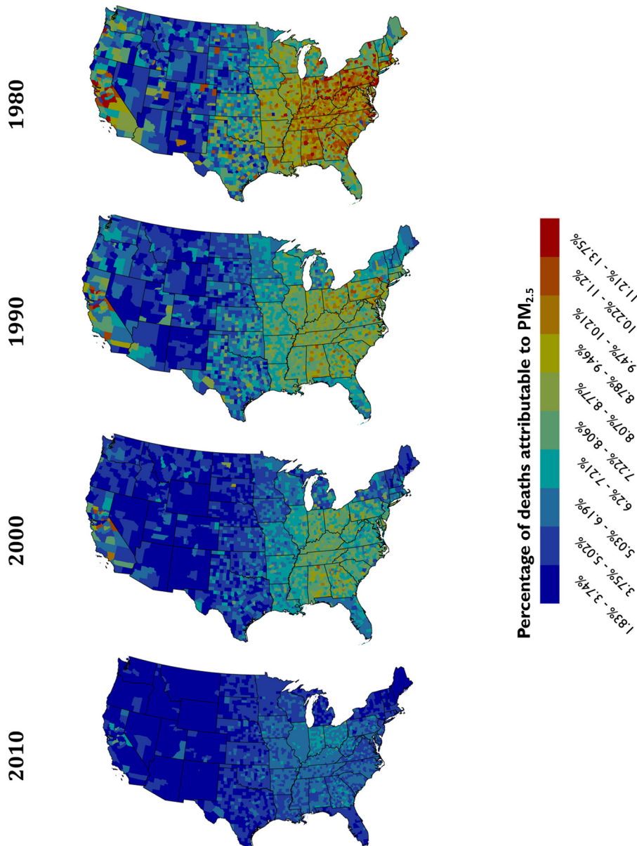
Figure 1. The fraction of total all-cause deaths attributable to PM 2.5 in U.S. counties in the years 1980, 1990, 2000, and 2010 among adults ages 30 and older (calculated using risk coefficient from Krewski et al. 2009). State and county boundaries for each year drawn according to Census Topologically Integrated Geographic Encoding and Referencing (TIGER)/Line files as reported by the Minnesota Population Center National Historical Geographic Information System (NHGIS Database) ( http://www.nhgis.org ).
