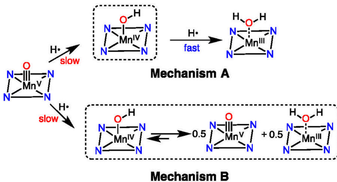
Scheme 2. Possible Mechanisms for H-atom Abstraction by an Mn V (O) Complex
