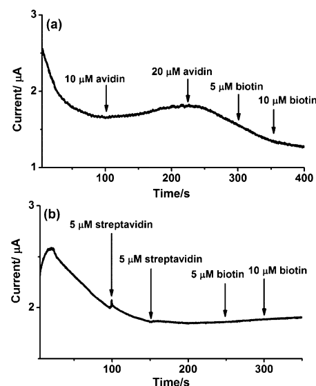
Figure 3. (a) i-t curve obtained following the sequential addition of avidin and biotin. (b) i-t curve obtained following the sequential addition of streptavidin and biotin. The detection was achieved on the Nafion-modified BDD electrode vs Ag/AgCl, the potential was at +1.8 V.
