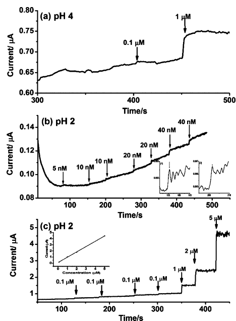
Figure 2. (a) i-t curve for LOD determination using 0.2 M acetate buffer, pH 4. (b) i-t curve for LOD determination using 0.2 M phosphate buffer, pH 2; 10 nM biotin [(b), insert]. (c) Calibration curve of biotin. The detection was achieved on the Nafion-modified BDD electrode vs Ag/AgCl, the potential was at +1.8 V, using 0.2 M phosphate buffer, pH 2.
