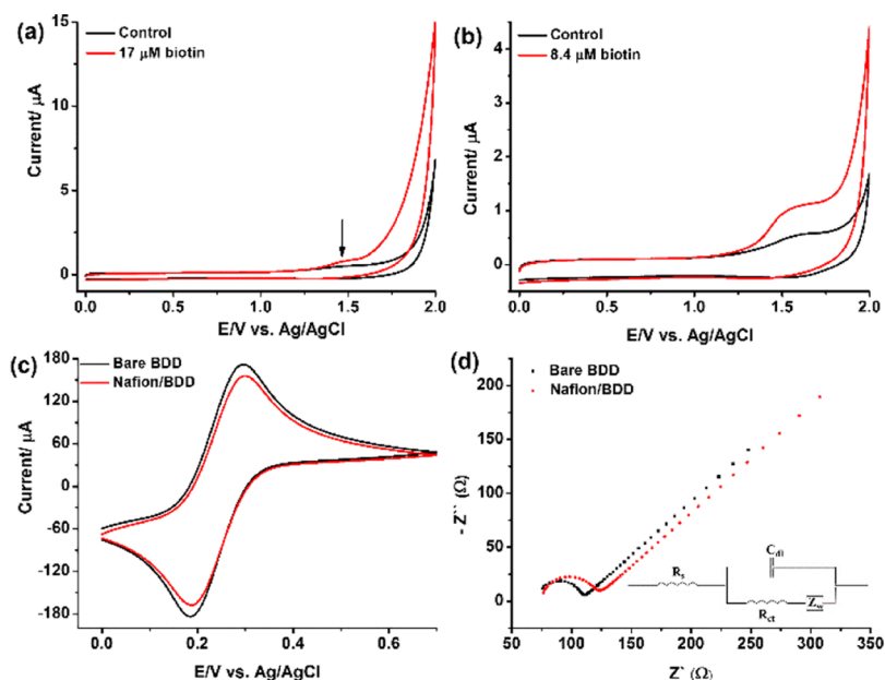
Figure 1. CVs of biotin obtained by the Nafion-modified BDD electrode vs Ag/AgCl using (a) 0.2 M acetate buffer, pH 4; (b) 0.2 M phosphate buffer, pH 2, a scan rate of 100 \text{ mV s}^{-1} ; (c) the CV of the bare and Nafion-modified BDD electrodes at a scan rate of 50 \text{ mV s}^{-1} and (d) EIS of the bare and Nafion-modified BDD electrodes (inset: the modified Randles circuit). \text{Fe}(\text{CN})_6^{4-/3-} (10 mM) prepared in 0.1 M KCl.
