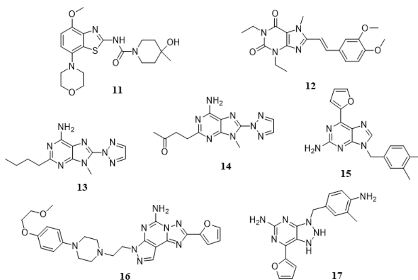
Fig. (3). Chemical structures of A 2A AR antagonists in clinical trials for PD treatment: SYN-115 or Tozadenant ( 11 ), KW-6002 or Istradefylline ( 12 ), ST1535 ( 13 ), ST4206 ( 14 ), BIIB014/V2006 ( 15 ), SCH-420814/MK-3814 or Preladenant ( 16 ), and V-81444 ( 17 ). The chemical structure of PBF-509 was not disclosed.
