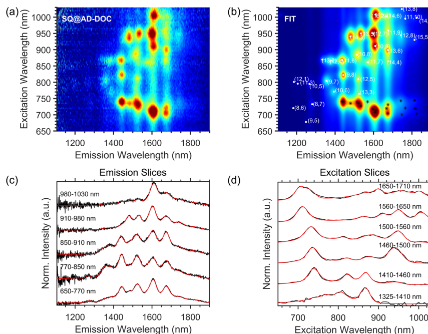
Figure 5. 2D spectral analysis PLE map of the SQ@AD-DOC sample. (a) Experimental PLE map of SQ@AD-DOC. (b) 2D fit of the PLE map, including both the intrinsic SWCNT PLE peaks (white dots) and the respective EET peaks (indicated by black stars). (c,d) Selected emission and excitation slices for the denoted excitation/emission wavelength ranges, showing the excellent correspondence between experimental data (black traces) and fit (red traces).
