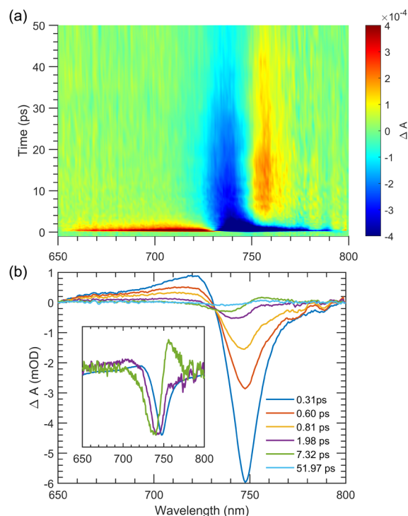
Figure 4. Focus on TA of the SQ@LV950-ATPE sample near the SQ absorption. (a) 2D TA map showing the spectral evolution of the encapsulated SQ absorption. (b) Selected TA spectra for short (sub-ps), medium (ps), and long (tens of ps) time scales. Inset shows a few selected normalized TA spectra (see also Figure S23 for kinetic slices at different probe wavelengths).
