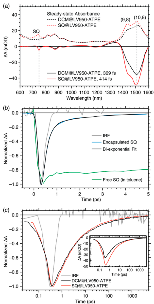
Figure 3. TA spectroscopy of ATPE-sorted LV950 SWCNTs pumped at 748 nm ( i.e. , in the SQ absorption band). (a) Peak transient absorption spectra at early times (solid traces) and steady-state absorption spectra (dashed traces) of DCM-filled (black traces) and SQ-filled (red traces) SWCNTs. Dashed vertical lines indicate the probe wavelengths at which the kinetic slices in panel b, that is, 748 nm (also the pump wavelength) and in panel c, that is, 1511 nm were obtained. (b) Kinetic slices for the SQ ground state bleach at 748 nm (blue trace), with the corresponding biexponential fit (black trace). The kinetic traces for free SQ dye in toluene (green trace) and the instrument response function, IRF (gray trace), are shown for reference. A probe-wavelength-dependent TA map is presented in Figure 4. (c) Kinetic slices at the peak (1511 nm) of the NIR ground state bleach dominated by the (10,8) S_{11} transition for the SQ@LV950-ATPE (red trace) and reference DCM@LV950-ATPE (black trace). The kinetic trace for the IRF (gray trace) is shown for reference. Inset: Non-normalized kinetics with same color scheme as main panel.
