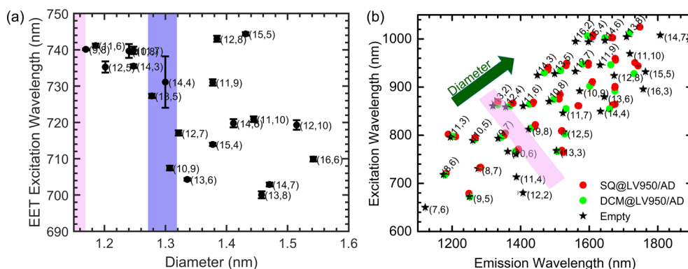
Figure 6. (a) Position of the EET excitation peak, extracted from the 2D spectral analysis of the dye-filled PLE maps, as a function of the s -SWCNT diameter. The pink shaded area (in both panels a and b) represents the minimal encapsulation diameter range, and the purple shaded area represents the diameter range after which a more complex behavior is found with the diameter of the SWCNTs increasing according to the green arrow in panel (b) (see also main text). (b) Peak positions of empty (black stars), SQ-filled (red circles), and DCM-filled (green circles) SWCNTs as obtained from the PLE fits. A clear change in S_{11}/S_{22} peak position between the SQ- and DCM-filled samples can be observed for SWCNTs with diameters similar or larger than the (9,8) SWCNT, indicative of filling with the SQ-molecules, also highlighted by the pink shaded area.
