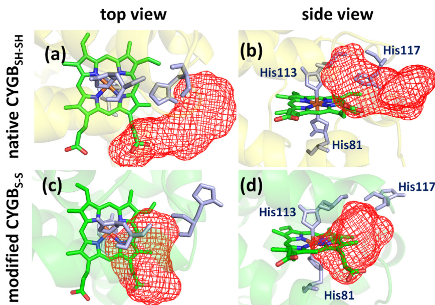
Fig. 6. Binding hot spots. Binding hot spot of \text{CYGB}_{\text{SH}\dots\text{SH}} (a-b) and (c-d) \text{CYGB}_{\text{S-S}} presented as red meshed regions. The helices in the structures are represented in pale colors, for the sake of clarity. The heme group and the histidine residues (81, 113, 117) are shown in green and light purple colors and licorice views, respectively. It is clear that in \text{CYGB}_{\text{SH}\dots\text{SH}} the access to the heme group is more limited than in \text{CYGB}_{\text{S-S}} .
