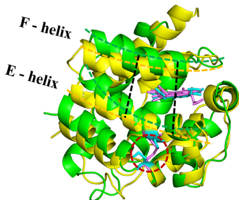
Fig. 5. Aligned structures of CYGB SH...SH (yellow) and CYGB S-S (green). The distances between Ala 88 -Ala 107 and Ala 82 -Ala 112 are depicted by black dashed lines. The yellow and green dashed lines are plotted to indicate shifted positions of the E- and F-helices. The heme group and cysteine residues of both CYGB SH...SH and CYGB S-S are presented in licorice view in blue and pink, respectively. The disulfide (S-S) bridge is shown within the red dashed circle.
