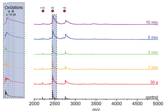
Fig. 4. Native MS after reduction with DTT. Native MS spectra of 10 \mu\text{M} CYGB in 100 mM ammonium acetate after adding 10 mM DTT. Monomeric +9 is highlighted. Inset: the zoomed in section of the monomeric +9 peak. Addition of DTT leads to a loss of the dimers via reduction of disulfide bridges. DTT also seems to reduce the number of oxidations (narrowing of the peaks). See also Fig. 2 for comparison.
