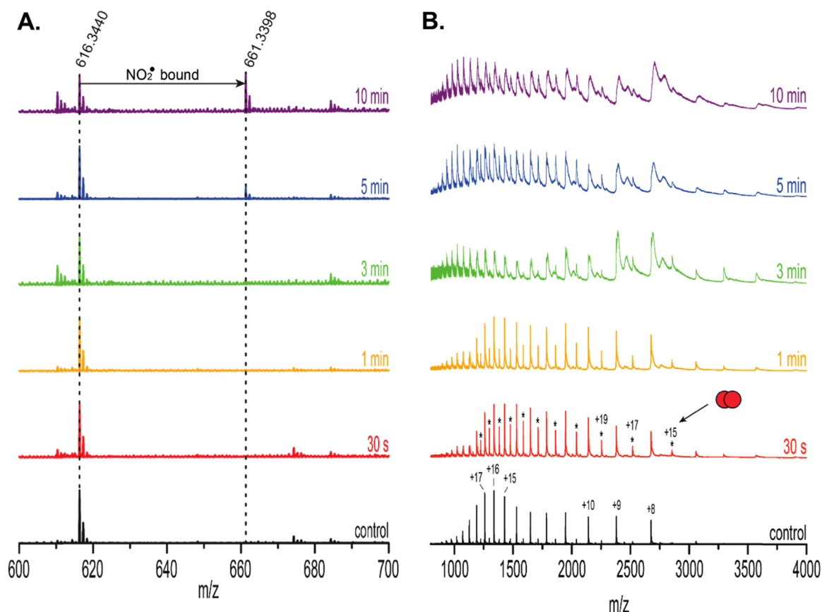
Fig. 3. Denaturing MS of CYGB. ESI spectra of 10 \mu\text{M} CYGB (diluted 1:1 in acetonitrile containing 1% formic acid) after different duration of plasma treatment (20 \mu\text{M} CYGB in 50 mM tris-buffer). (A.): Zoomed in m/z region from 600 to 700. The peak at 616.3440 m/z represents the free heme group. 5–10 min of treatment induces binding of a molecule, i.e. \text{NO}_2 to the heme group (661.3398 m/z ). (B.): Full spectrum ranging from 800 to 4000 m/z showing the apo-form of the protein. The appearance of smaller peaks (asterisks) in between the monomers highlights the presence of covalent dimers in the sample. The theoretical mass of CYGB in the apo-form (without heme) is 21 404.62 Da compared to the experimental mass of 21 407.29 \pm 4.16 Da in the control.
