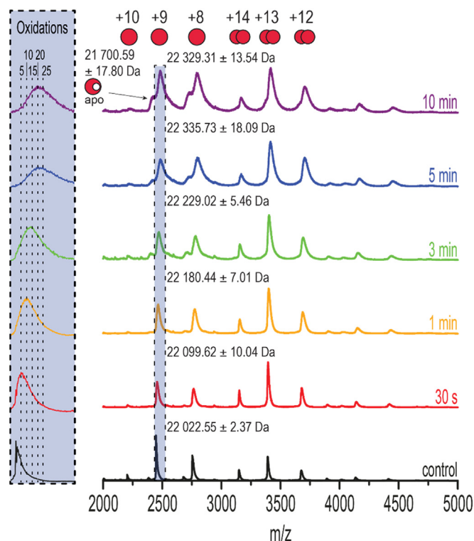
Fig. 2. Native MS. Native MS spectra of 10 \mu M holo CYGB in 100 mM ammonium acetate after different duration of plasma treatment (20 \mu M CYGB in 50 mM tris-buffer). Monomeric (+10, +9, +8) and dimeric (+14, +13, +12) species are identified. The monomeric +9 species are highlighted in blue. Inset: zoomed in section of the +9 monomers, highlighting mass shifts and peak broadening caused by plasma-induced oxidations. The theoretical mass of holo CYGB is 22,021.11 Da.
