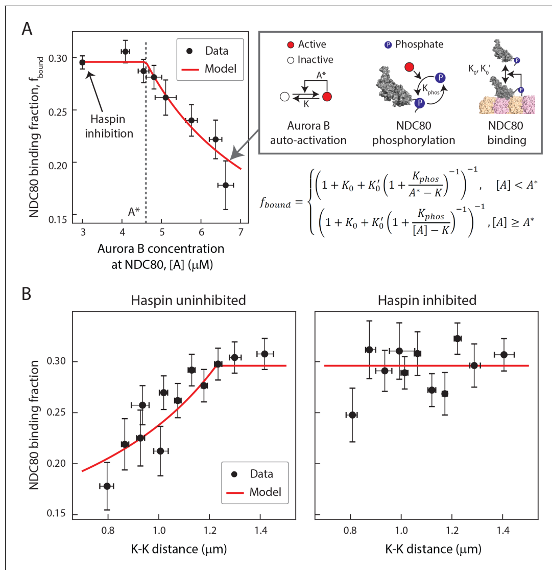
Figure 7. A biophysical model of tension dependent NDC80-kMT binding. (A) Plot of NDC80 binding fraction, f_{bound} , (converted from NDC80 FRET fraction in Figures 3D and 5E ) vs. Aurora B concentration at NDC80, [A] (converted from INCENP-mCherry intensity in Figure 6B , see Materials and methods). Data points (black circles) are the mean and SEM. We constructed a mathematical model that predicts NDC80 binding fraction from Aurora B concentration at NDC80 through three steps: intermolecular Aurora B auto-activation, NDC80 phosphorylation, and NDC80-kMT binding. Red line shows the mathematical model fit to the data. (B) NDC80 binding fraction vs. K-K distance before (left) and after (right) haspin inhibition by 5-ITu. The data points (black circles) are adapted from Figures 3D and 5E . Red lines are the predictions from the mathematical model. Data points are available in Figure 7-Data (Yoo et al., 2018).
