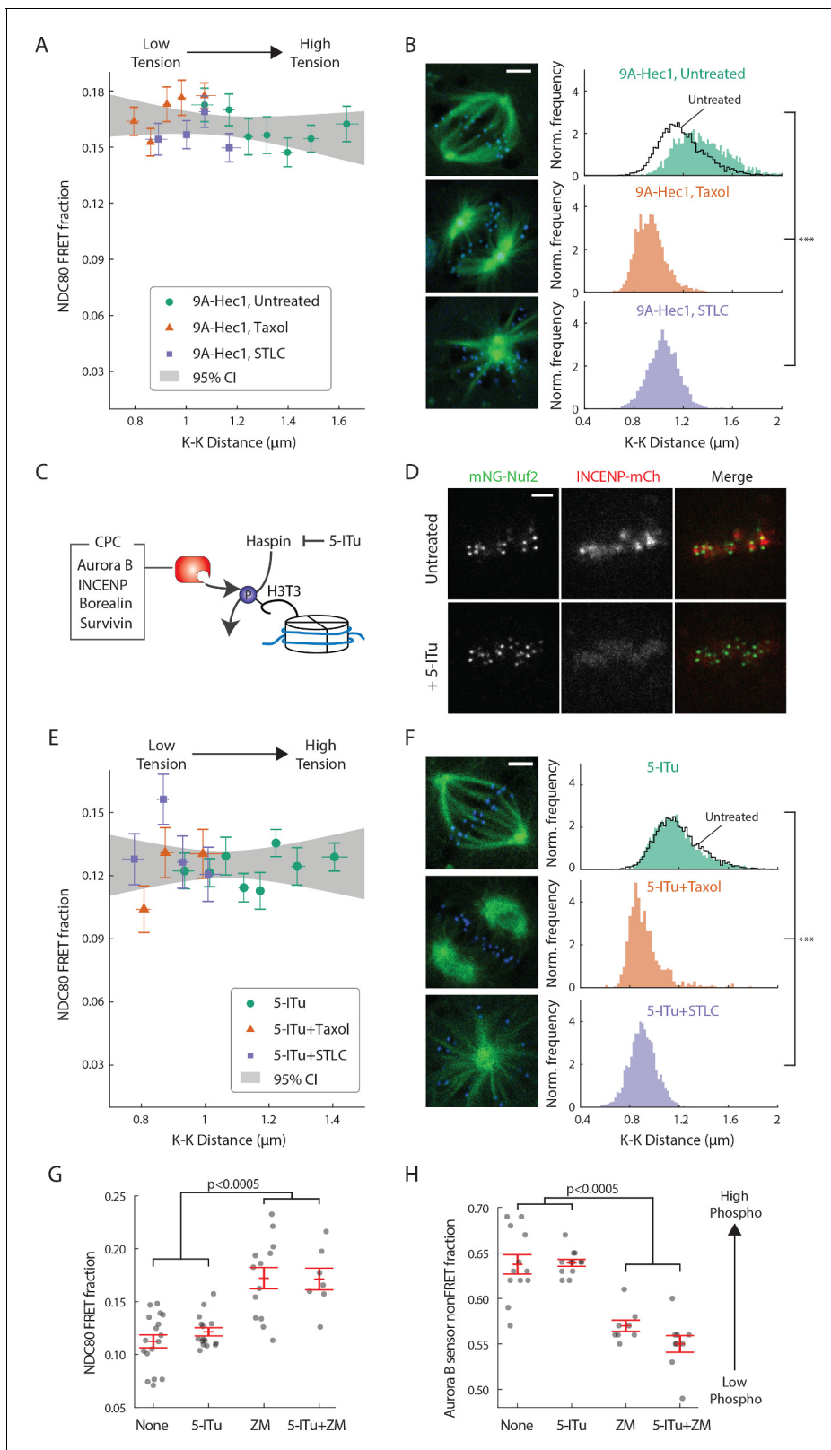
Figure 5. Haspin-dependent centromere-localized Aurora B is responsible for the tension dependency of NDC80-KMT binding. (A) NDC80 FRET fraction vs. K-K distance for 9A-Hec1-expressing cells with no drug treatment (green circle, n = 12 cells, 803 kinetochores/data point), with 10 \mu\text{M} taxol treatment (orange triangle, n = 9 cells, 1113 kinetochores/data point), or with 5 \mu\text{M} STLC treatment (purple square, n = 10 cells, 855 kinetochores/data point). For STLC data, only poleward-facing kinetochores are included (see Figure 5—figure supplement 1A for comparison between poleward-facing kinetochores and non-poleward-facing kinetochores). (B) Representative fluorescence images and histograms of NDC80 FRET fraction for 9A-Hec1 cells under Untreated, Taxol, and STLC conditions. (C) Schematic of the CPC complex (Aurora B, INCENP, Borealin, Survivin) and its interaction with Haspin, H3T3, and 5-ITu. (D) Representative fluorescence images of mNG-Nuf2, INCENP-mCh, and Merge for Untreated and +5-ITu cells. (E) NDC80 FRET fraction vs. K-K distance for 5-ITu treated cells under low to high tension. (F) Representative fluorescence images and histograms of NDC80 FRET fraction for 5-ITu treated cells under Untreated, Taxol, and STLC conditions. (G) NDC80 FRET fraction for different treatments (None, 5-ITu, ZM, 5-ITu+ZM) with p < 0.0005 . (H) Aurora B sensor nonFRET fraction for different treatments (None, 5-ITu, ZM, 5-ITu+ZM) with p < 0.0005 , showing a shift towards high phosphorylation.
