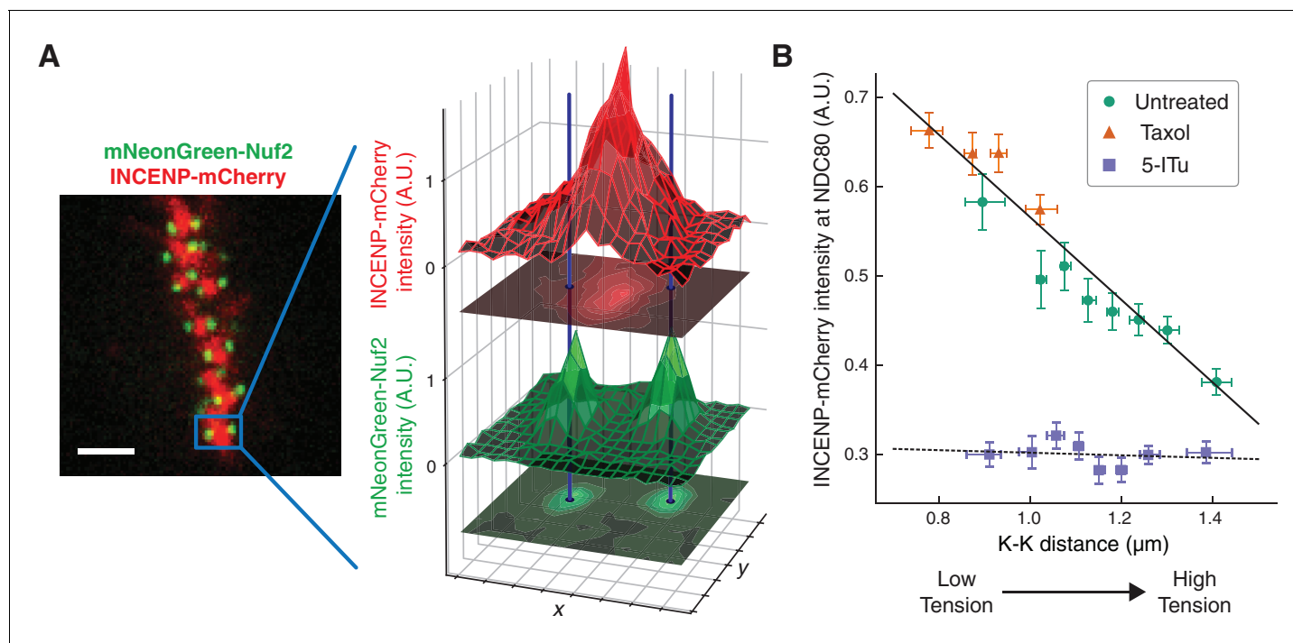
Figure 6. The concentration of Aurora B at the location of NDC80 decreases with centromere tension. (A) Spinning-disk confocal microscopy image of mNeonGreen-Nuf2 (green) and INCENP-mCherry (red). 3 \mu\text{m} scale bar. The location of NDC80 was determined to sub-pixel accuracy, using the mNeonGreen-Nuf2 image. For each pair of sister kinetochores, the intensity of INCENP-mCherry at the location of NDC80 was measured and normalized on a cell-by-cell basis. (B) Normalized INCENP-mCherry intensity at the location of NDC80 were averaged within groups of kinetochores with similar K-K distances, and plotted against the K-K distances for untreated (green circles), taxol-treated (orange triangles), and 5-ITu-treated (purple squares) cells. Data points are the mean, y-error bars the SEM, and the x-error bars the interquartile ranges. Black solid and dotted lines are the linear fits to DMSO+taxol combined data and 5-ITu data, respectively. 906 kinetochore pairs in 9 cells, 599 pairs in 8 cells, and 680 pairs in 6 cells were analyzed for DMSO control, taxol treatment, and 5-ITu treatment data, respectively. Data points and source FLIM data are available in Figure 6-Data (Yoo et al., 2018).
