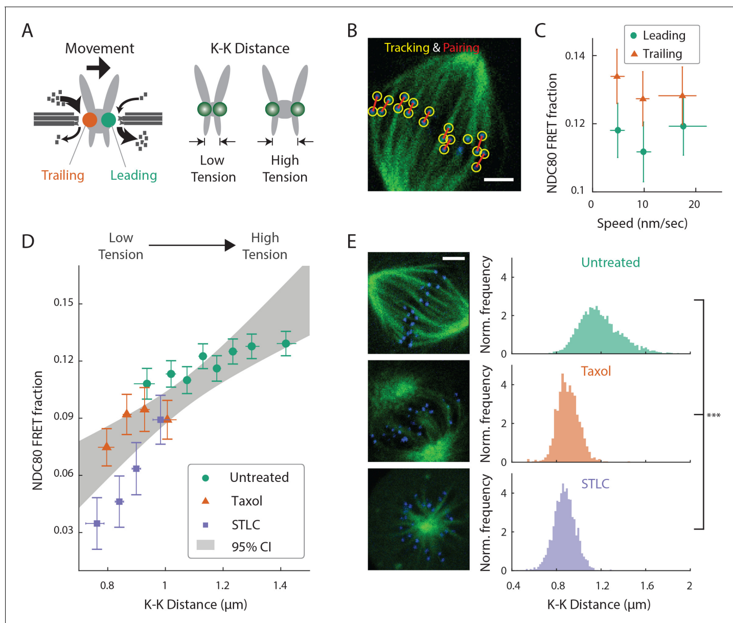
Figure 3. NDC80-kMT binding is correlated with kMT dynamics and centromere tension. (A) (left) kMTs predominantly depolymerize at leading kinetochores and polymerize at trailing kinetochores. (right) K-K distance is a proxy for centromere tension. Measuring NDC80-kMT binding along with the kinetochore movement and K-K distance therefore reveals how NDC80-kMT binding is related to the kMT dynamics and centromere tension. (B) Image of a metaphase cell with mTurquoise2-NDC80 (blue) and \beta -tubulin-TC-FIAsH (green), and kinetochore tracking (yellow circles) and pairing (red lines) results. 3 \mu\text{m} scale bar. (C) NDC80 FRET fraction vs. kinetochore speed for leading (green circle) and trailing (orange triangle) kinetochores ( n = 17 cells, 681 kinetochores/data point). Data points are the mean, y-error bars the SEM, and the x-error bars the interquartile ranges within groups of kinetochores with similar velocities. (D) NDC80 FRET fraction vs. K-K distance for untreated cells (green circle, n = 17 cells, 984 kinetochores/data point), cells treated with 10 \mu\text{M} taxol (orange triangle, n = 7 cells, 525 kinetochores/data point), and cells treated with 5 \mu\text{M} STLC (purple square, n = 16 cells, 493 kinetochores/data point). For STLC data, only poleward-facing kinetochores are plotted (see Figure 3—figure supplement 2 for comparison between poleward and anti-poleward kinetochores). Data points are the mean, y-error bars the SEM, and the x-error bars the interquartile ranges within groups of kinetochores with similar K-K distances. Gray area is the 95% confidence interval for the linear fit to the combined data. (E) Histograms of K-K distances for the untreated (top, green), taxol-treated (middle, orange), and STLC-treated (bottom, purple) cells. 3 \mu\text{m} scale bar in the cell images of mTurquoise2-NDC80 (blue) and beta-tubulin-TC-FIAsH (green). ***p-value (Welch's t-test) less than 10^{-30} . Data points and source FLIM data are available in Figure 3-Data (Yoo et al., 2018).
