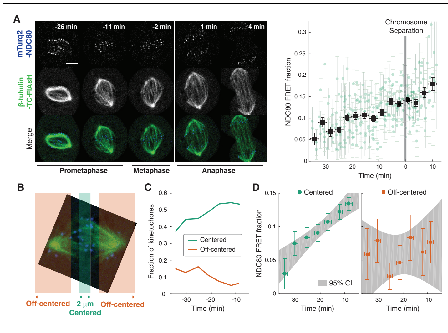
Figure 2. NDC80-kMT binding is regulated in a chromosome-autonomous fashion. (A) Example cell images and time course of NDC80 FRET fraction from prometaphase to metaphase to anaphase ( n = 11 cells). Black squares are the mean, y-error bars are the SEM, and x-error bars are the SD of the data points (green circles) in equally spaced time intervals. 5 \mu\text{m} scale bar. (B) Kinetochores at each time point in prometaphase cells are divided into two groups, centered and off-centered, based on their distances from the metaphase plate. Kinetochores less than 1 \mu\text{m} away from the metaphase plate were classified as centered, and kinetochores more than 2.5 \mu\text{m} away were classified as off-centered. (C) Time course of the fraction of centered (green) and off-centered (orange) kinetochores in prometaphase. (D) Time course of NDC80 FRET fraction of centered (green circles) and off-centered (orange squares) kinetochores in prometaphase ( n = 11 cells, 2886 centered and 572 off-centered kinetochores). Data points are the mean, y-error bars the SEM, and the x-error bars the SD in equally spaced time intervals. Gray areas are the 95% confidence intervals for the linear fits. Data points and source FLIM data are available in Figure 2-Data (Yoo et al. , 2018).
