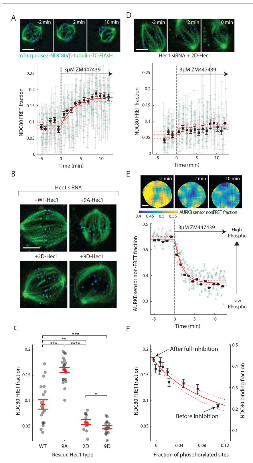
Figure 4. Aurora B kinase regulates NDC80-kMT binding in a graded fashion in vivo. (A) (top) Cell images showing mTurquoise2-NDC80 (blue) and beta-tubulin-TC-FIAsH (green). (bottom) Time course of NDC80 FRET fraction in response to Aurora B inhibition by 3 \mu M ZM447439 (n = 15 cells). (B) Images of cells with mTurquoise2-NDC80 (blue) and beta-tubulin-TC-FIAsH (green) after depleting endogenous Hec1 by siRNA and expressing siRNA-insensitive WT or three different phosphomimetic mutants of Hec1: 9A-, 2D-, and 9D-Hec1 (see Materials and methods). (C) NDC80 FRET fraction of Figure 4 continued on next page
