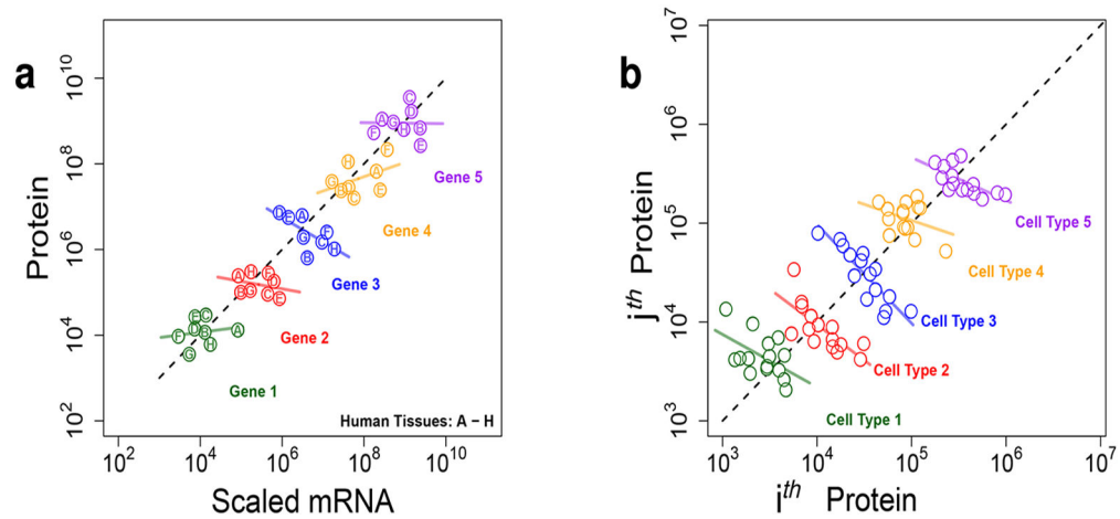
Figure 2. Simpson’s paradox confounds the interpretation of population-average protein and mRNA measurements. (a) For a particular gene, its protein levels across tissues can be poorly predicted by its mRNA levels, whereas the average protein levels can be well predicted by scaled mRNA levels. 19 Thus mRNAs levels are unreliable surrogates for relative protein levels, and we need direct measurements of proteins. (b) Related manifestation of Simpson’s paradox indicates that the average levels of the i th and the j th proteins may appear positively correlated, even though they are inversely correlated within a cell type. Averaging across cells, even cell types sorted based on markers, will obscure the relationship between the i th and the j th proteins.
